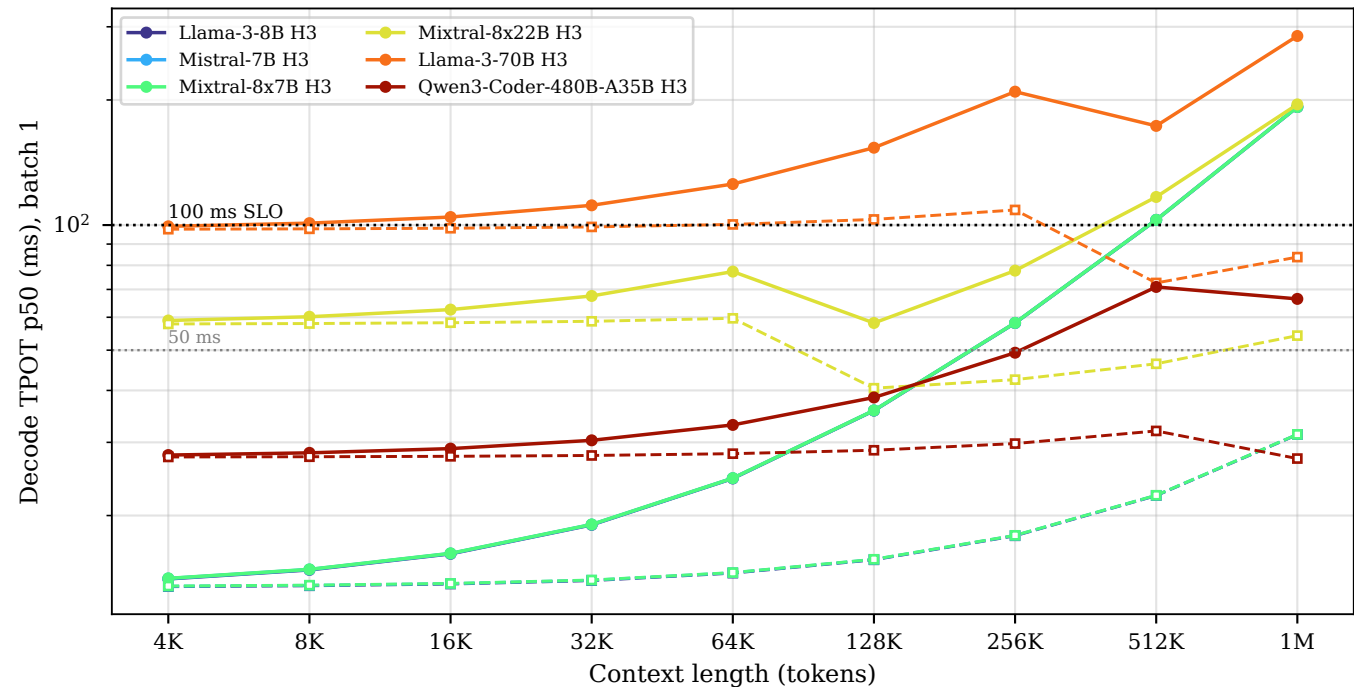
Decode latency vs context: H3 (solid) vs SPLASH (dashed) — Blackwell
