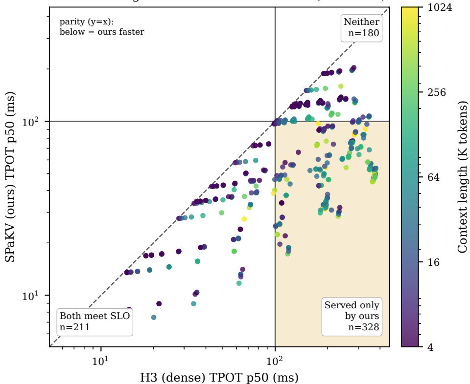
All 719 configs vs the 100 ms TPOT SLO (Blackwell)
