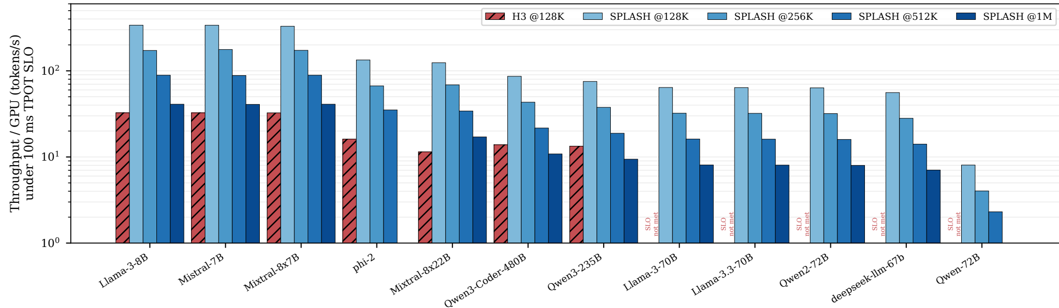
Sustainable decode throughput per GPU ( \div TP), H3 vs SPLASH, long contexts — Blackwell
