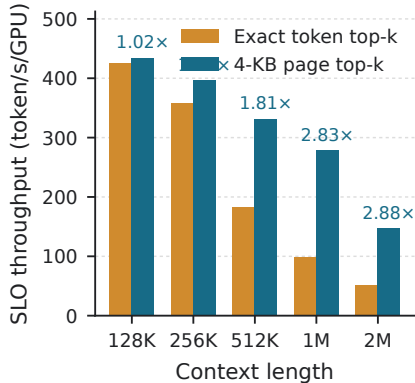
(a) Same 10% logical token budget
