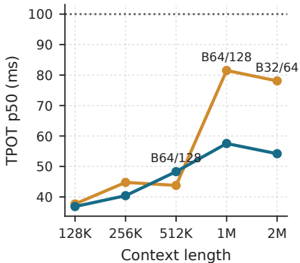
(b) Independently selected batch
