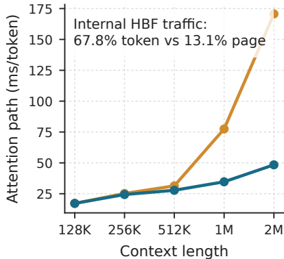
(c) Fixed batch=64
