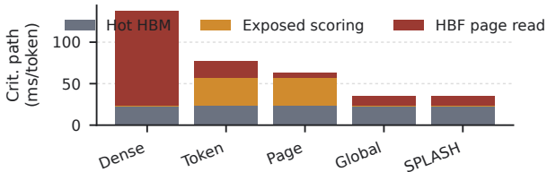
(a) Where attention latency goes at 1M
