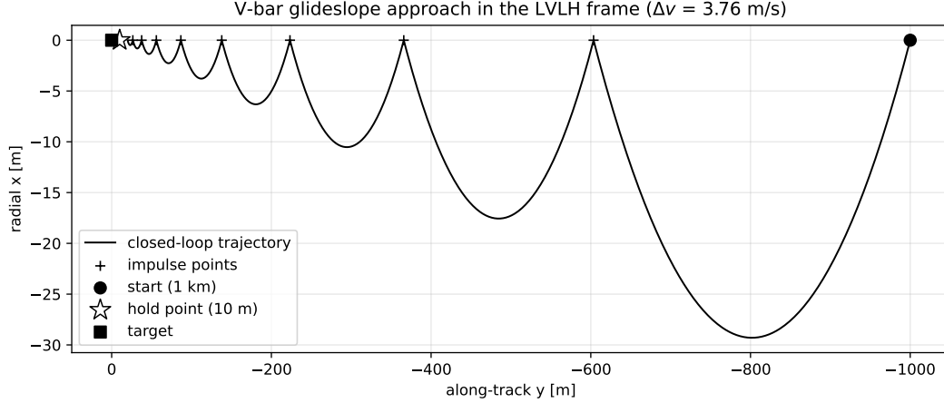
Figure 3: Trajectory of the vbar_approach.py demo: a 1 km V-bar glideslope approach to a 10 m hold point in the local-vertical/local-horizontal (LVLH) frame, planned on the Clohessy–Wiltshire discretization and propagated under the linear Clohessy–Wiltshire dynamics. The verified pipeline (nonlinear truth model, temporal-logic checks, and the exact barrier) is the reference mission, exercised in continuous integration rather than by this demo; the exact-rational KKT checker runs as a separate checker test.
