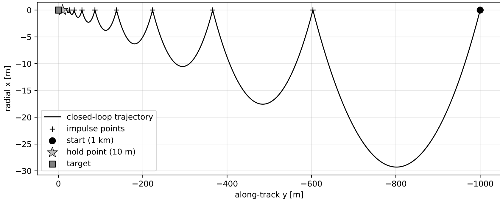
V-bar glideslope approach in the LVLH frame ( \Delta v = 3.76 m/s)
