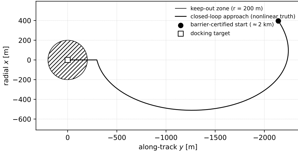
Figure 3: Reference mission: the closed-loop rendezvous approach from the barrier-certified start set ( \approx 2 km) to the docking target under the nonlinear relative-motion truth model, in the local vertical/local horizontal (LVLH) frame. The transfer keeps clear of the keep-out zone and completes on the docking corridor; the passive-abort safety of the start set is certified in exact rational arithmetic by the barrier.
