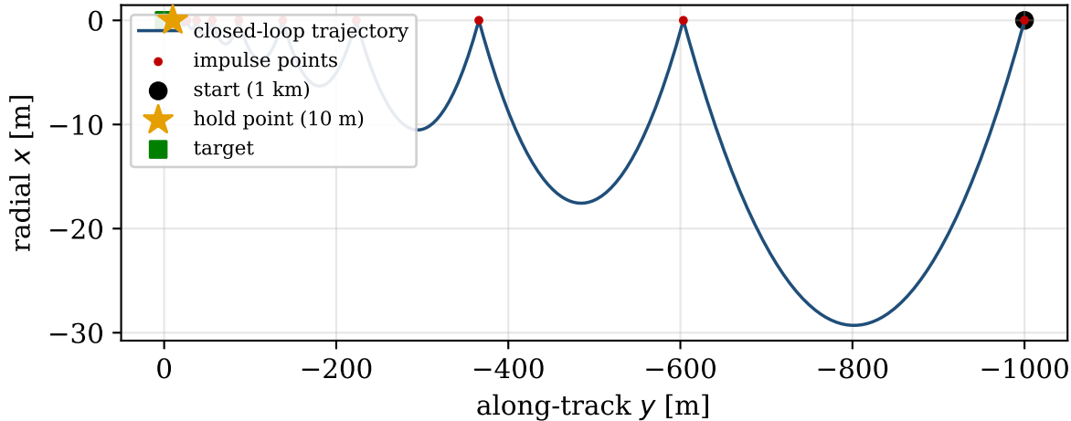
V-bar glideslope approach in the LVLH frame ( \Delta v = 3.76 m/s)
