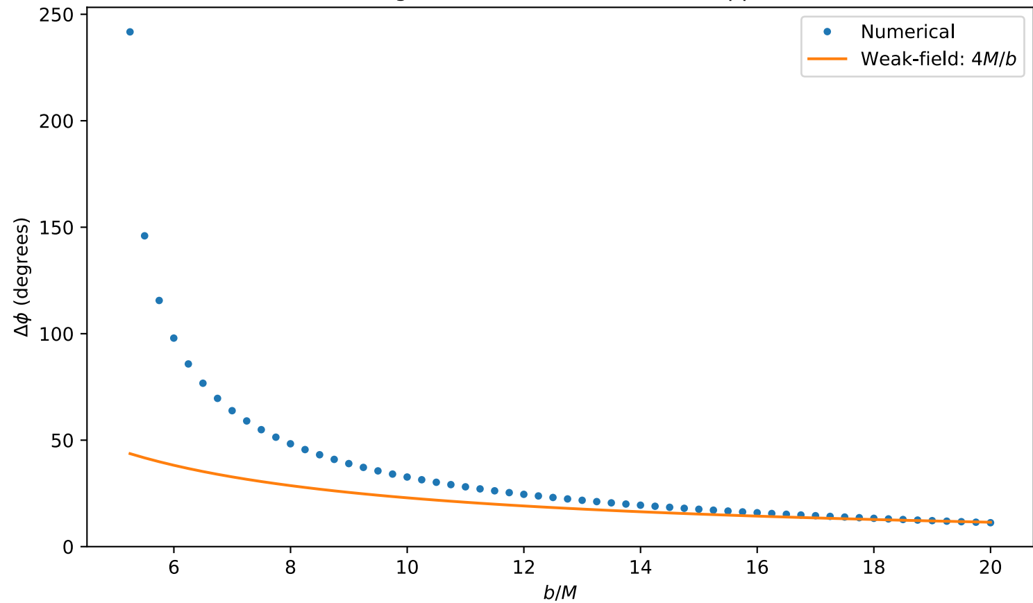
Deflection angle: numerical vs weak-field approximation
