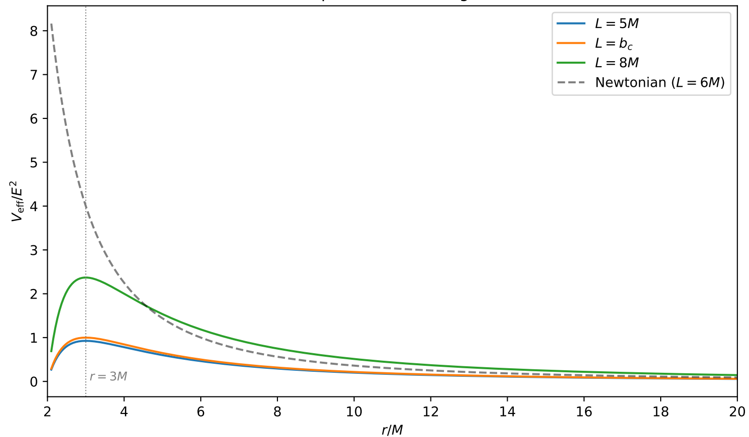
Effective potential for null geodesics
