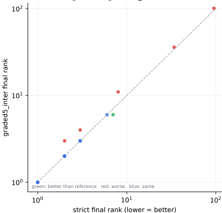
Final target rank: graded5_inter vs strict (all)
