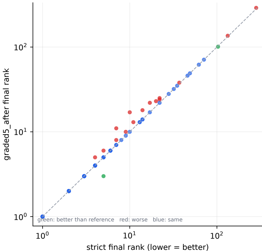
Final target rank: graded5_after vs strict (last)
