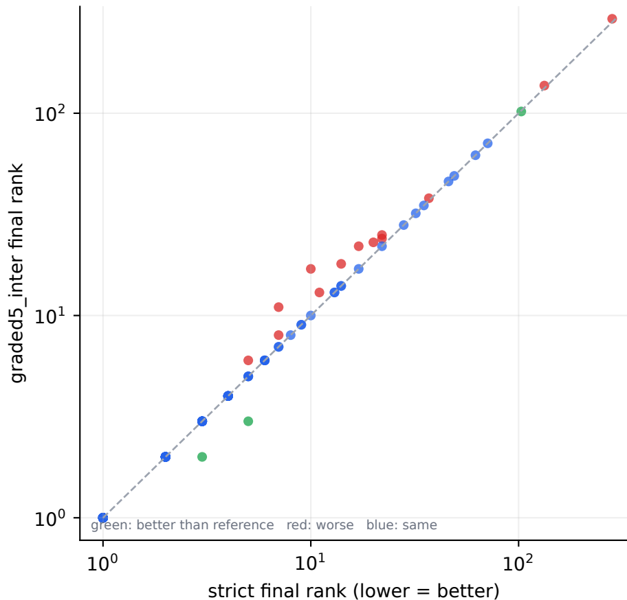
Final target rank: graded5_inter vs strict (last)
