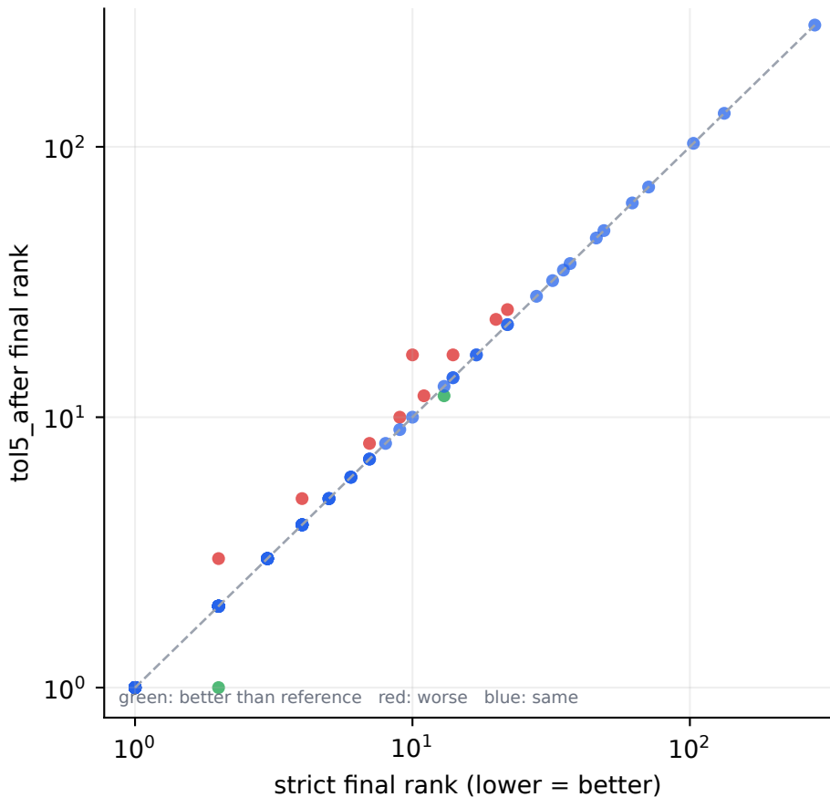
Final target rank: tol5_after vs strict (last)
