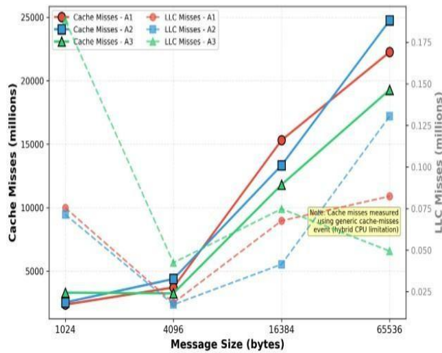
Plot 3: Cache Behavior vs Message Size (4 Threads)
