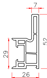
112 SCREEN SASH TRACK Code: T112SSGD THK WT 2.0 0.54
