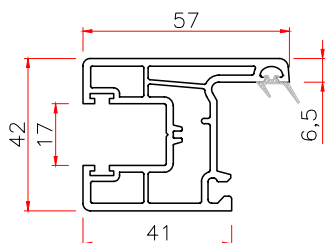
8857 SLIDING SASH
