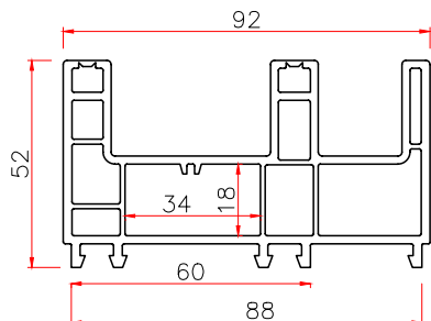
921 SLIDING FRAME Code: T921K THK WT 2.2 1.40 2.5 1.48
