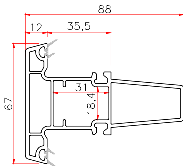
88 MULLION Code: T88ZT THK WT 2.2 1.23 2.5 1.33
