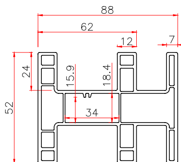
88 DOUBLE SLIDING FRAME
