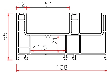
108 SLIDING FRAME Code: T108K THK WT 2.2 1.60 2.5 1.80
