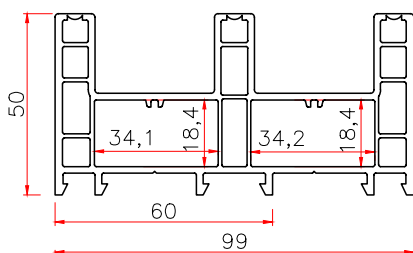
99 SLIDING FRAME Code: T99K THK WT 2.0 1.50 2.2 1.61
