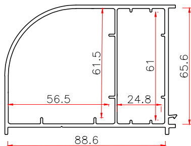
6588 BAY CORNER ADAPTOR Code: 6588ZJ WT 1.30
