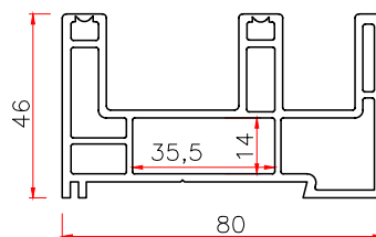
8046 SLIDING FRAME Code: T8046K THK WT 2.2 1.17
