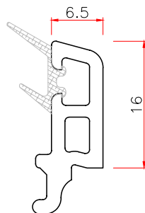
6.5 GLAZING BEAD Code: 6.5YT WT 0.170
