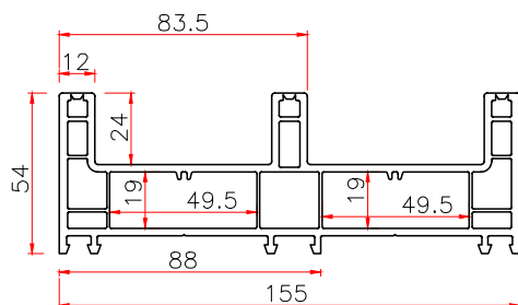
155 SLIDING FRAME
