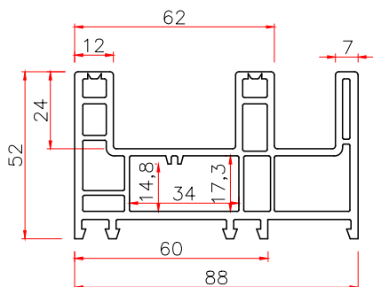
881 SLIDING FRAME Code: T881K THK WT 2.0 1.31 2.2 1.40 2.5 1.50
