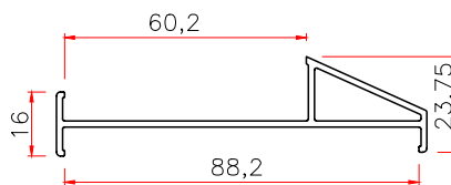
6088 FLAT BOARD Code: 6088PT WT 0.45
