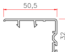
95 COVER
