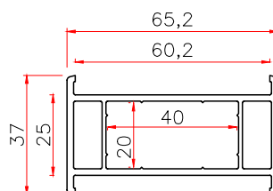
60 TUBE ADAPTOR Code: 60PG WT 0.68
