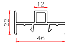
92 INTERLOCK Code: T92DJFB WT 0.41
