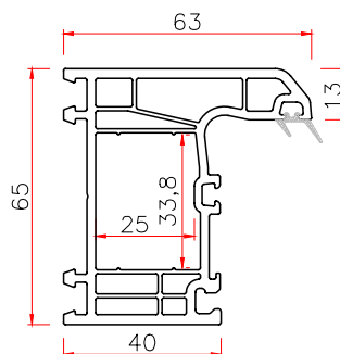
652 CASEMENT FRAME Code: P652K THK WT 2.5 1.28
