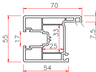
10870 SLIDING SASH Code: T10870S THK WT 2.2 1.25 2.5 1.37
