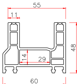
6055 SLIDING FRAME Code: T6055K THK WT 1.8 0.85 2.0 0.88
