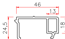
60 SHUTTER BEAD
