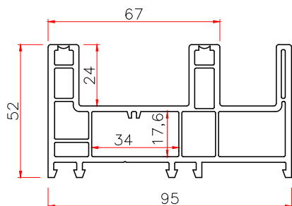
951 SLIDING FRAME
