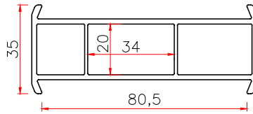
80 BAY CORNER ADAPTOR Code: T80ZJ WT 1.04
