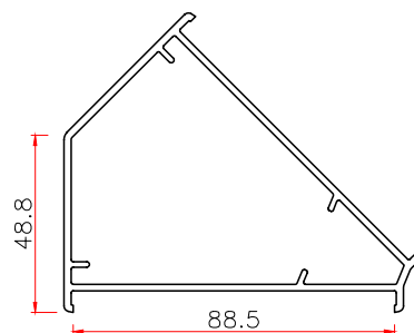
882 BAY CORNER ADAPTOR
