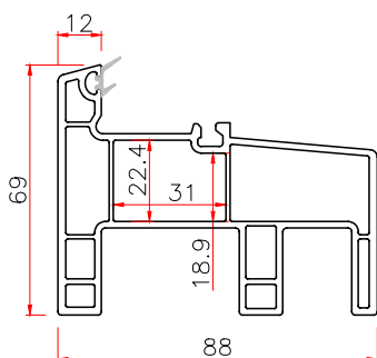
881 CONNECTED FRAME
