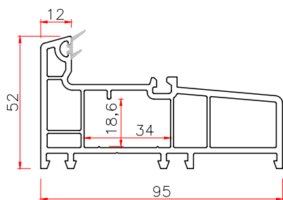
95 FIXED FRAME
