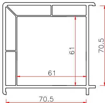
70 BAY CORNER ADAPTOR
