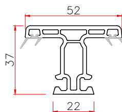
80 SASH MULLION Code: T80SZT THK WT 2.0 0.75
