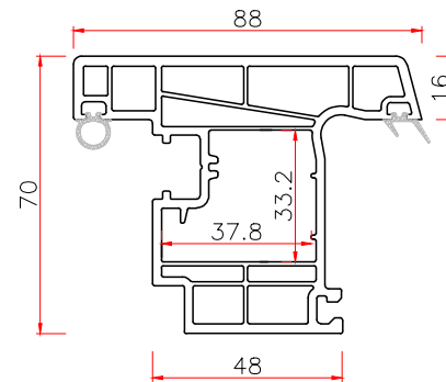
70 OUTWARD SASH
