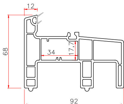
922 CONNECTED FRAME Code: T922LTK THK WT 2.2 1.58
