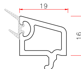
19 GLAZING BEAD Code: 19YT WT 0.219
