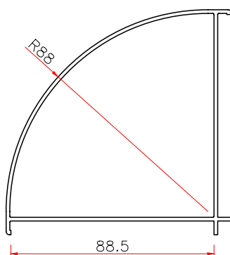
881 BAY CORNER ADAPTOR
