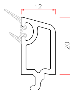
12 GLAZING BEAD Code: 12YT WT 0.220
