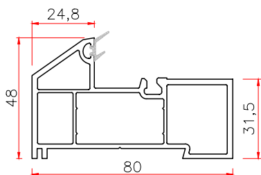
801 FIXED FRAME Code: T801GDK THK WT 2.2 0.99
