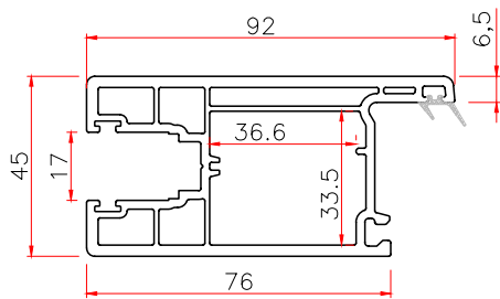
9292 DOOR SASH Code: T9292MS THK WT 2.5 1.60
