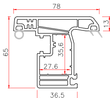
652 OUTWARD SASH Code: P652WS THK WT 2.5 1.50
