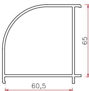
60 BAY CORNER ADAPTOR Code: 60ZJ WT 0.71
