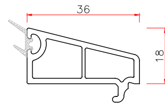
36 GLAZING BEAD Code: 36YT WT 0.342
