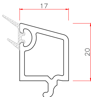
17 GLAZING BEAD Code: 17YT WT 0.257
