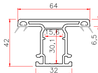
88 SASH MULLION
