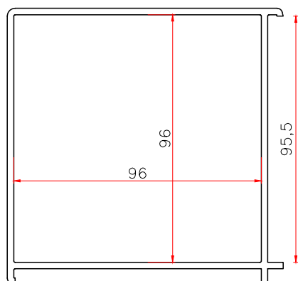
95 BAY CORNER
