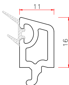
11 GLAZING BEAD Code: 11YT WT 0.207
