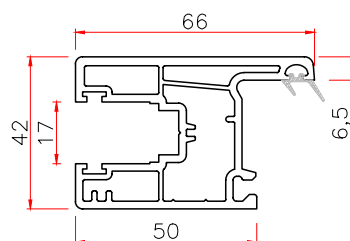
8866 SLIDING SASH
