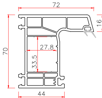
70 CASEMENT FRAME
