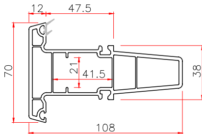
108 MULLION Code: T108ZT THK WT 2.5 1.63
