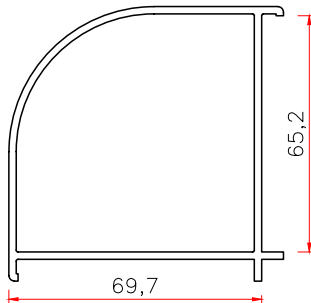
65 BAY CORNER ADAPTOR Code: 65ZJ WT 0.90
