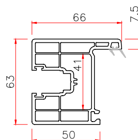
12066 SLIDING SASH
