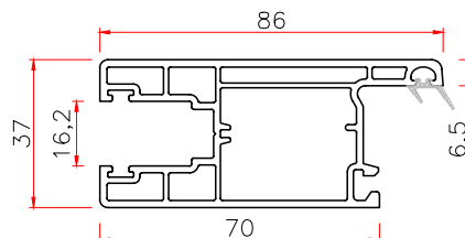
8086 SLIDING SASH Code: T8086S THK WT 1.8 1.20 2.3 1.28
