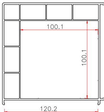
120 BAY CORNER
