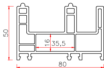
80502 SLIDING FRAME Code: T80502K THK WT 2.2 1.33
