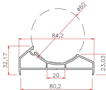
80 ANY ANGLE CORNER ADAPTOR Code: 80RYZZ BASE WT 0.73
