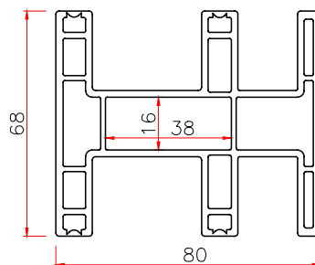
80 DOUBLE SLIDING FRAME Code: T80WZK THK WT 2.0 1.65
