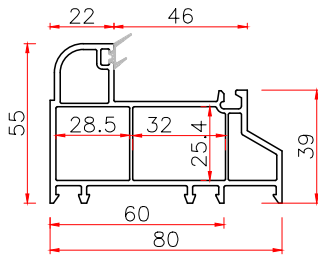
80 BR FRAME Code: P80K-BR THK WT 2.0 0.96
