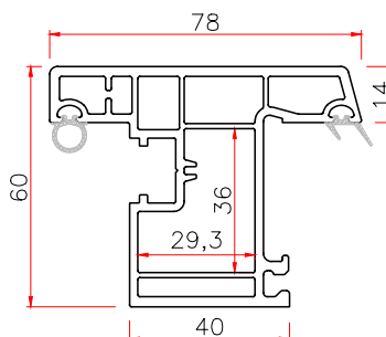
601 OUTWARD SASH
