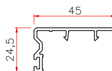
882 COVER Code: T882FG WT 0.23
