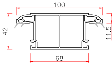
80 BR MULLION Code: P80ZT-BR THK WT 2.0 1.02
