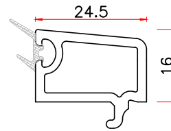
24.5 GLAZING BEAD Code: 24.5YT WT 0.260
