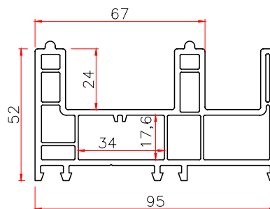
951 SLIDING FRAME
