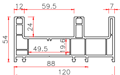
120 SLIDING FRAME
