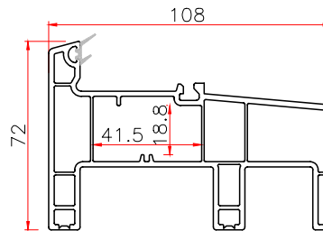
108 CONNECTED FRAME Code: T108LTK THK WT 2.2 1.73
