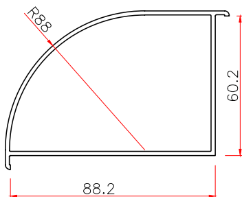
6088 BAY CORNER ADAPTOR Code: 6088ZJ WT 0.81
