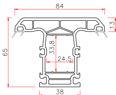
652 MULLION Code: P652ZT THK WT 2.5 1.47
