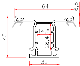
92 SASH MULLION Code: T92SZT THK WT 2.2 0.97
