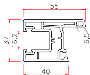
8055 SLIDING SASH Code: T8055S THK WT 2.0 0.785 2.2 0.83
