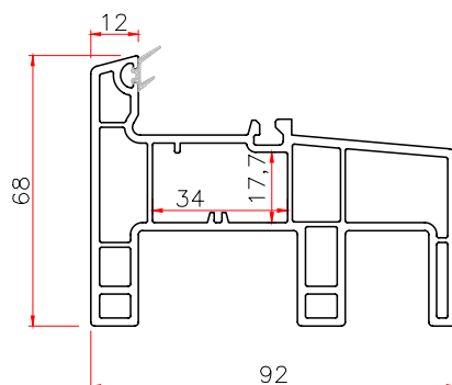
921 CONNECTED FRAME Code: T921LTK THK WT 2.2 1.52 2.5 1.72
