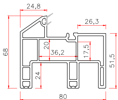
801 CONNECTED FRAME Code: T801LTK THK WT 2.0 1.46
