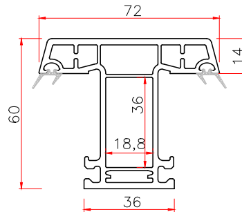
60 MULLION
