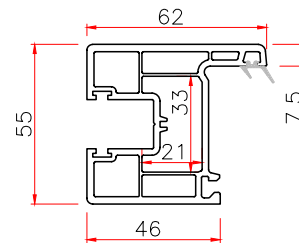
10870 SLIDING SASH Code: T10870S THK WT 2.2 1.25 2.5 1.37
