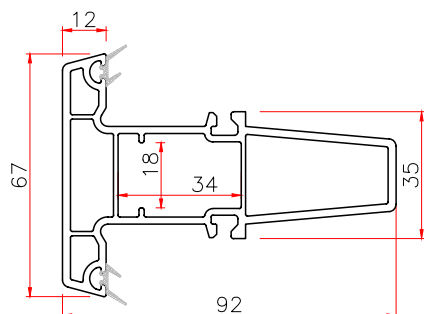
92 MULLION Code: T92ZT THK WT 2.2 1.25 2.5 1.37
