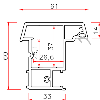
60 LAP JOINT Code: P60FZT THK WT 2.5 1.065
