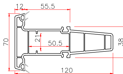
120 SLIDING FRAME
