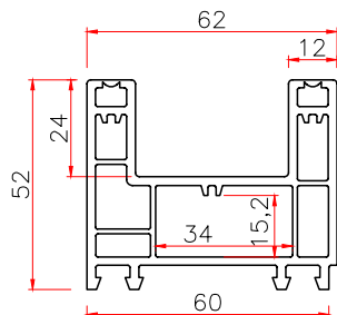
6062 SLIDING FRAME Code: T6062K THK WT 1.8 1.03 2.0 1.05 2.2 1.09
