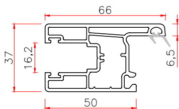
8066 SLIDING SASH Code: T8066S THK WT 1.8 0.88 2.0 0.91
