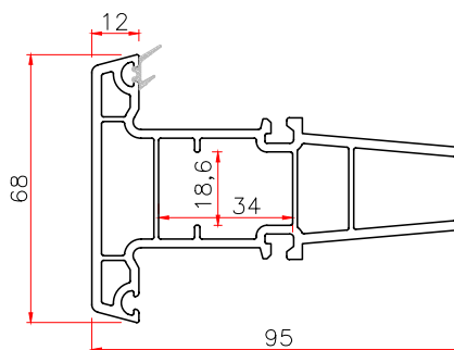
95 FIXED FRAME
