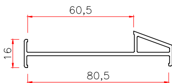
6080 FLAT BOARD Code: 6080PT WT 0.41
