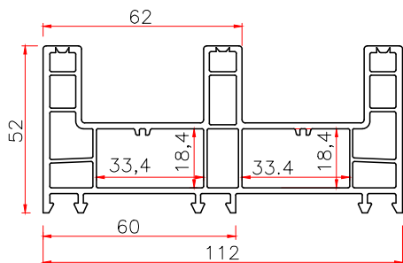
112 SLIDING FRAME Code: T112K THK WT 2.2 1.70
