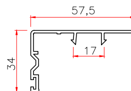
1081 COVER Code: T1081FG WT 0.30
