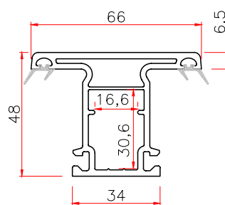
95 SASH MULLION
