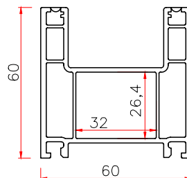
6060 SLIDING FRAME Code: T6060K THK WT 2.0 1.09 2.2 1.13 2.5 1.19
