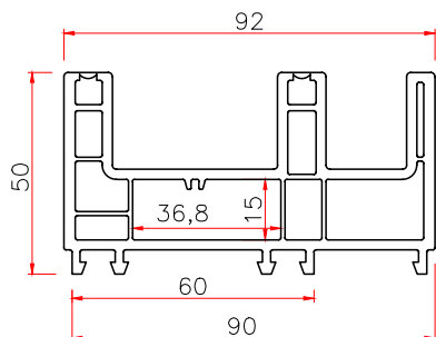
923 SLIDING FRAME Code: T923K THK WT 2.8 1.82
