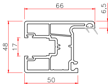
9566 SLIDING SASH
