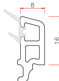
8 GLAZING BEAD Code: 8YT WT 0.181
