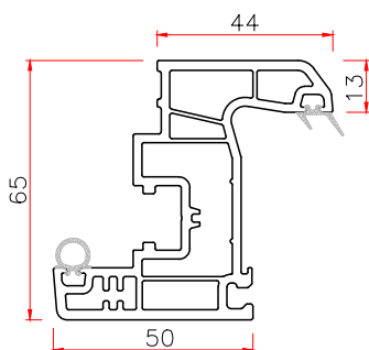
651 INWARD SASH Code: P651NS THK WT 2.5 1.30
