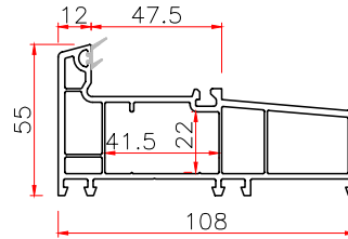
108 SLIDING FRAME Code: T108K THK WT 2.2 1.60 2.5 1.80
