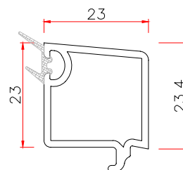
23 GLAZING BEAD Code: 23YT WT 0.290
