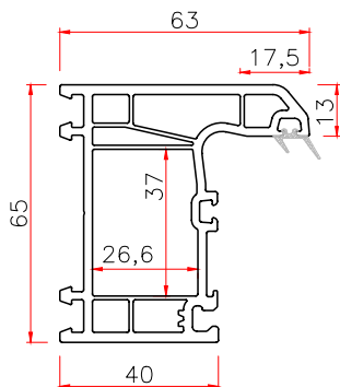
651 CASEMENT FRAME Code: P651K THK WT 2.5 1.20
