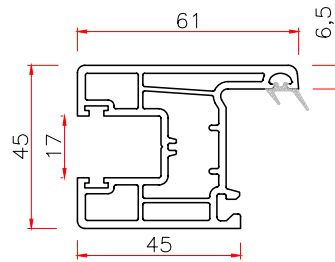
9261 SLIDING SASH Code: T9261S THK WT 2.2 1.00 2.5 1.07
