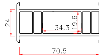
70 TUBE ADAPTOR
