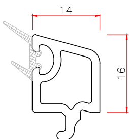
14 GLAZING BEAD Code: 14YT WT 0.216
