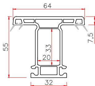
108 SASH MULLION Code: T108SZT THK WT 2.5 1.08
