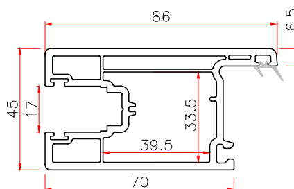
9286 DOOR SASH Code: T9286MS THK WT 2.8 1.65
