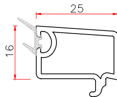
2516 GLAZING BEAD Code: 25YT-16 WT 0.270
