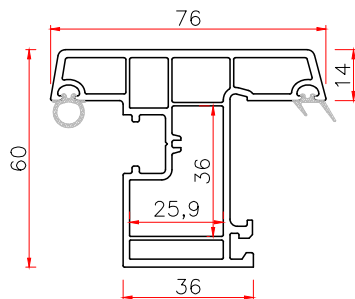
602 OUTWARD SASH
