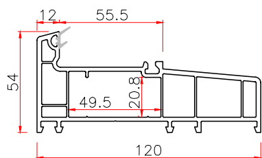
120 FIXED FRAME
