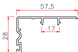
1082 COVER Code: T1082FG WT 0.28
