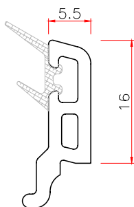
5.5 GLAZING BEAD Code: 5.5YT WT 0.135
