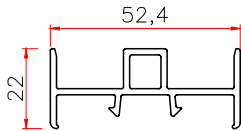
95 INTERLOCK Code: T95DJFB WT 0.44
