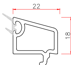
22 GLAZING BEAD Code: 22YT WT 0.258
