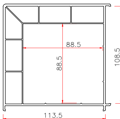
108 BAY CORNER ADAPTOR Code: T108ZJ WT 1.87
