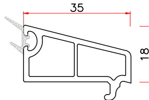
3518 GLAZING BEAD Code: 35YT-18 WT 0.317
