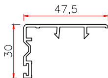
92 COVER Code: T92FG WT 0.25
