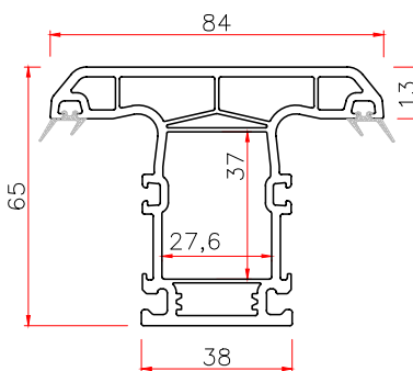
651 CASEMENT FRAME Code: P651K THK WT 2.5 1.20
