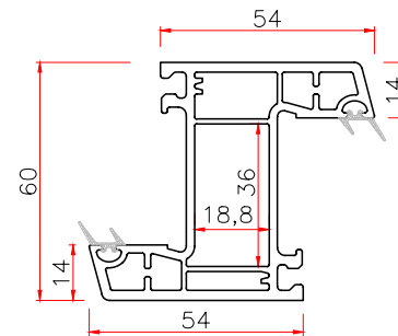
602 OUTWARD SASH
