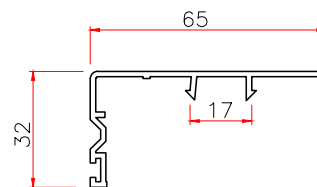
120 COVER
