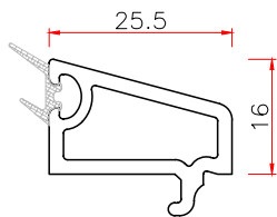
25.5 GLAZING BEAD Code: 25.5YT WT 0.261
