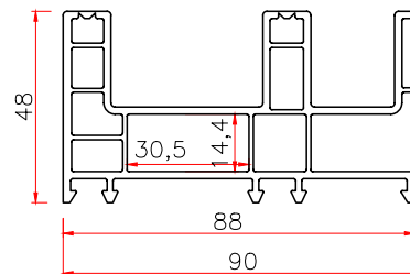
90 SLIDING FRAME Code: T90K THK WT 2.0 1.31
