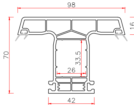
70 CASEMENT FRAME
