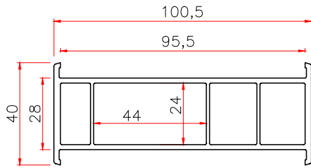
95 TUBE ADAPTOR Code: T95PG WT 1.15
