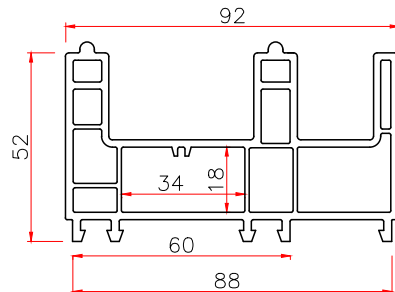
922 SLIDING FRAME Code: T922K THK WT 2.2 1.46 2.5 1.57
