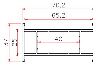
65 TUBE ADAPTOR Code: P65PG WT 0.75
