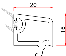
20 GLAZING BEAD Code: 20YT-16 WT 0.223
