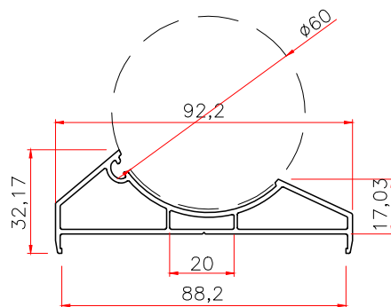
88 ANY ANGLE CORNER ADAPTOR Code: 88RYZZ BASE WT 0.83
