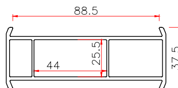
88 TUBE ADAPTOR
