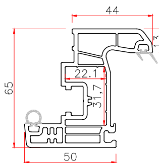
652 MULLION Code: P652ZT THK WT 2.5 1.47
