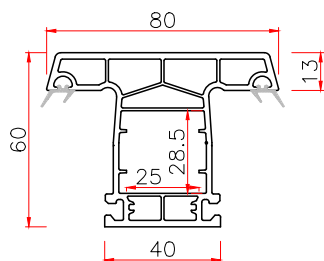
60T MULLION Code: P60ZT-T THK WT 2.2 1.30
