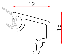
19 GLAZING BEAD Code: 19YT WT 0.219
