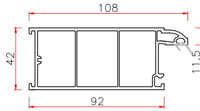
80 BR DOOR SASH Code: P80MS-BR THK WT 2.0 1.07
