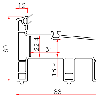
882 CONNECTED FRAME
