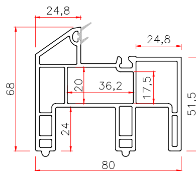
802 CONNECTED FRAME Code: T802LTK THK WT 2.0 1.50
