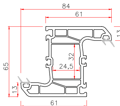
652 OUTWARD SASH Code: P652WS THK WT 2.5 1.50
