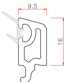
9.5 GLAZING BEAD Code: 9.5YT WT 0.196
