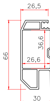
66 SCREEN SASH Code: T66SS THK WT 1.7 0.67
