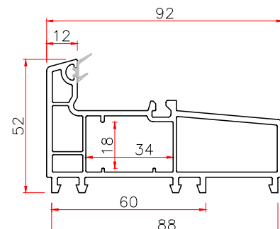
92 FIXED FRAME Code: T92GDK THK WT 2.2 1.15 2.5 1.25
