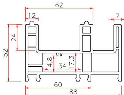
882 SLIDING FRAME Code: T882K THK WT 2.2 1.45
