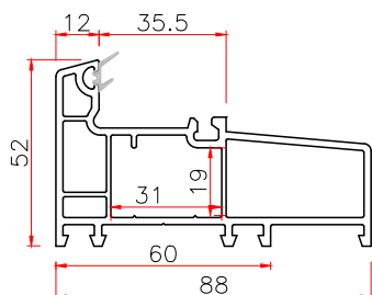
88 FIXED FRAME
