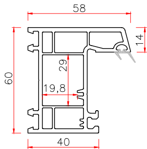
60 CASEMENT FRAME
