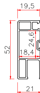
52 SCREEN SASH Code: T52SS THK WT 1.3 0.41 1.7 0.47
