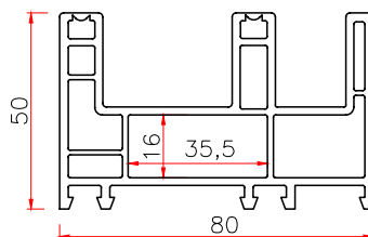
80501 SLIDING FRAME Code: T80501K THK WT 1.8 1.18 2.0 1.26 2.2 1.31
