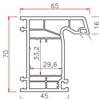
70 FIXED FRAME
