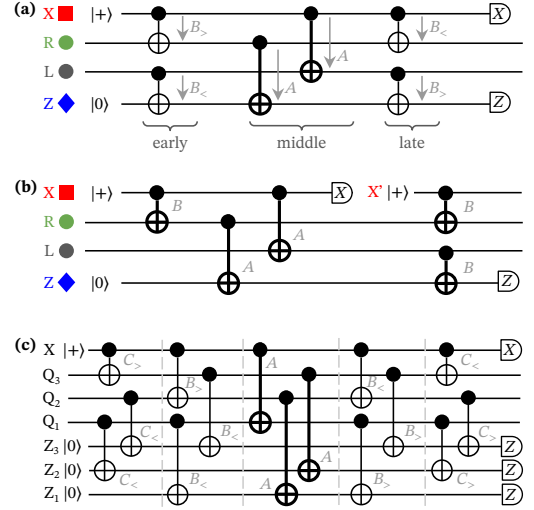
Figure 3: (a) Three-stage schedule for QALP codes. Each drawn CNOT represents a group of physical CNOTs; thick symbols apply all colors of \tilde{A} , while thin symbols apply half of the colors of \tilde{B} , denoted B_< (first half) and B_> (second half). (b) Pipelined multi-round schedule: half of the X-check gates in the next round overlap with half of the Z-check gates in the current round. (c) Five-stage schedule for 3D QALP codes.
