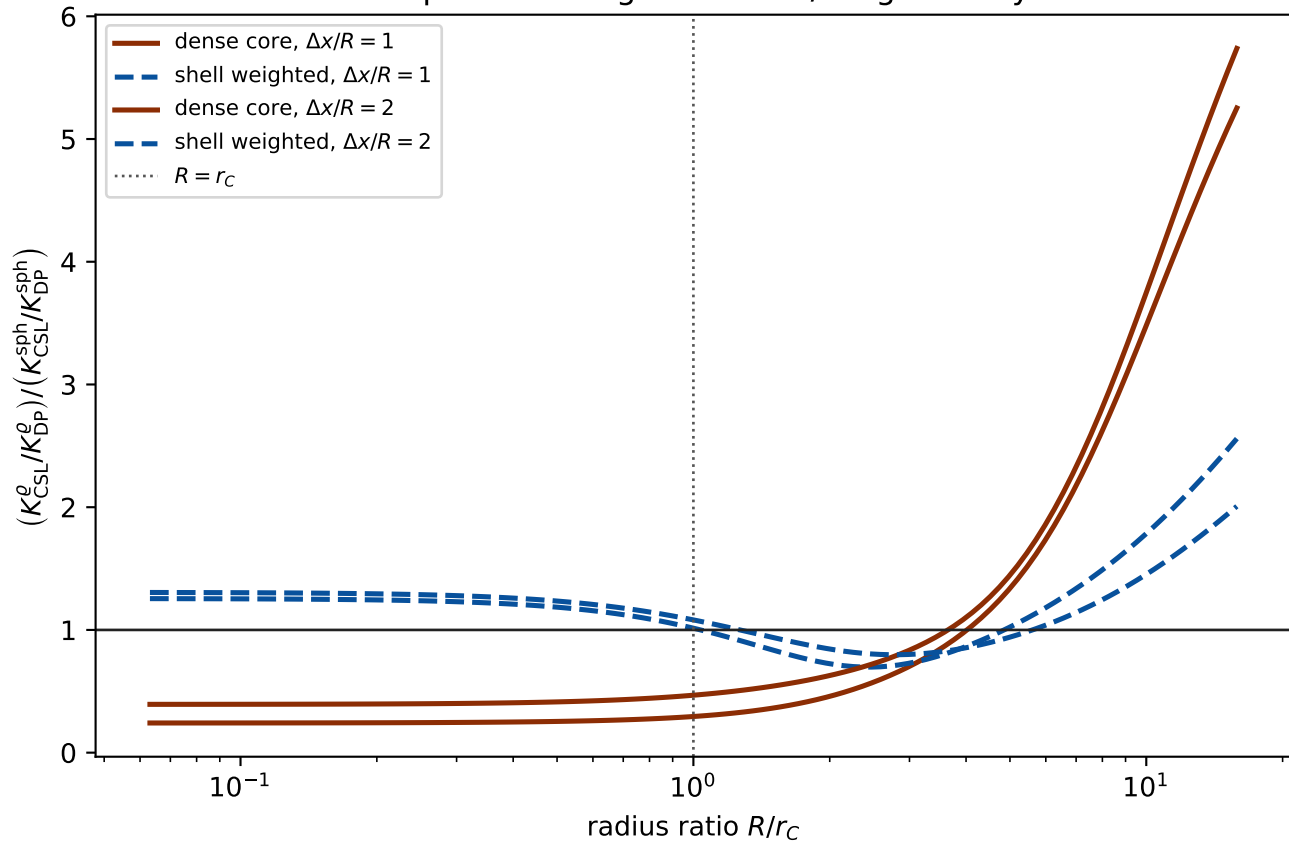
Core-shell profile tuning of the CSL/DP geometry factor
