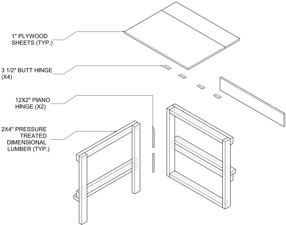
③ ASSEMBLY 1/2" = 1'0"
