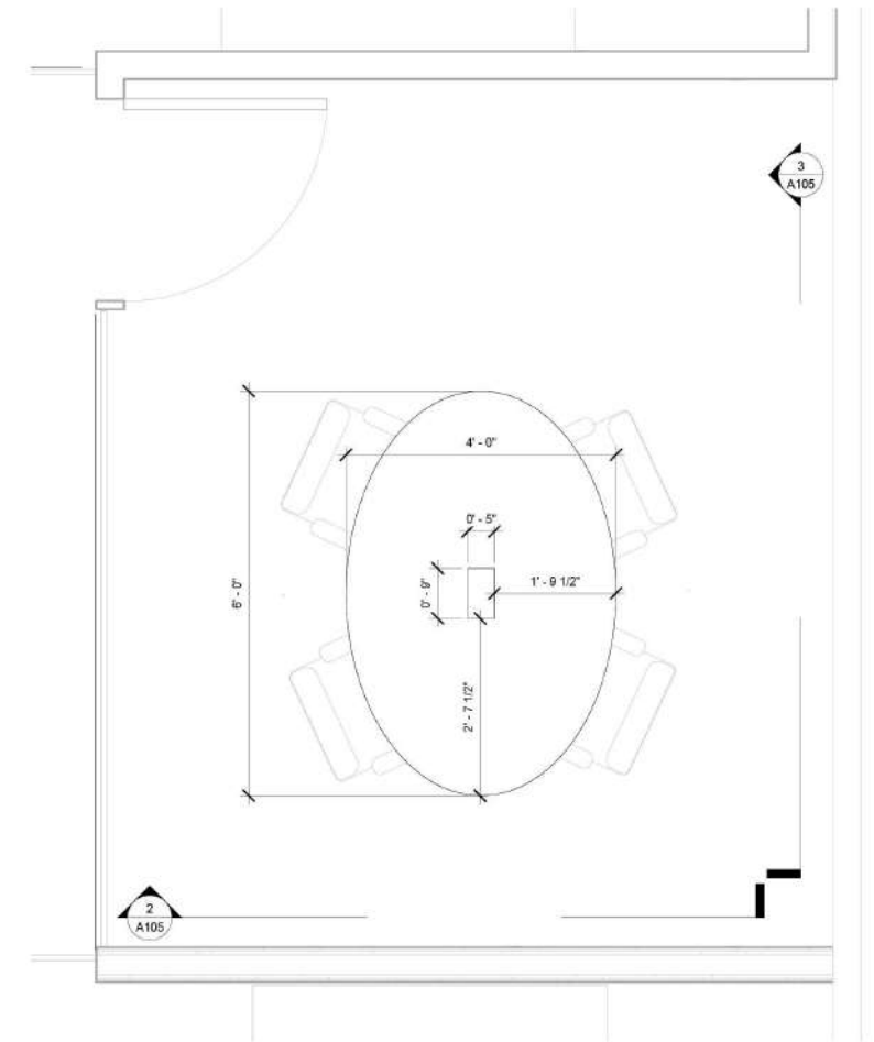
① Conference Table 3/4" = 1'-0"
