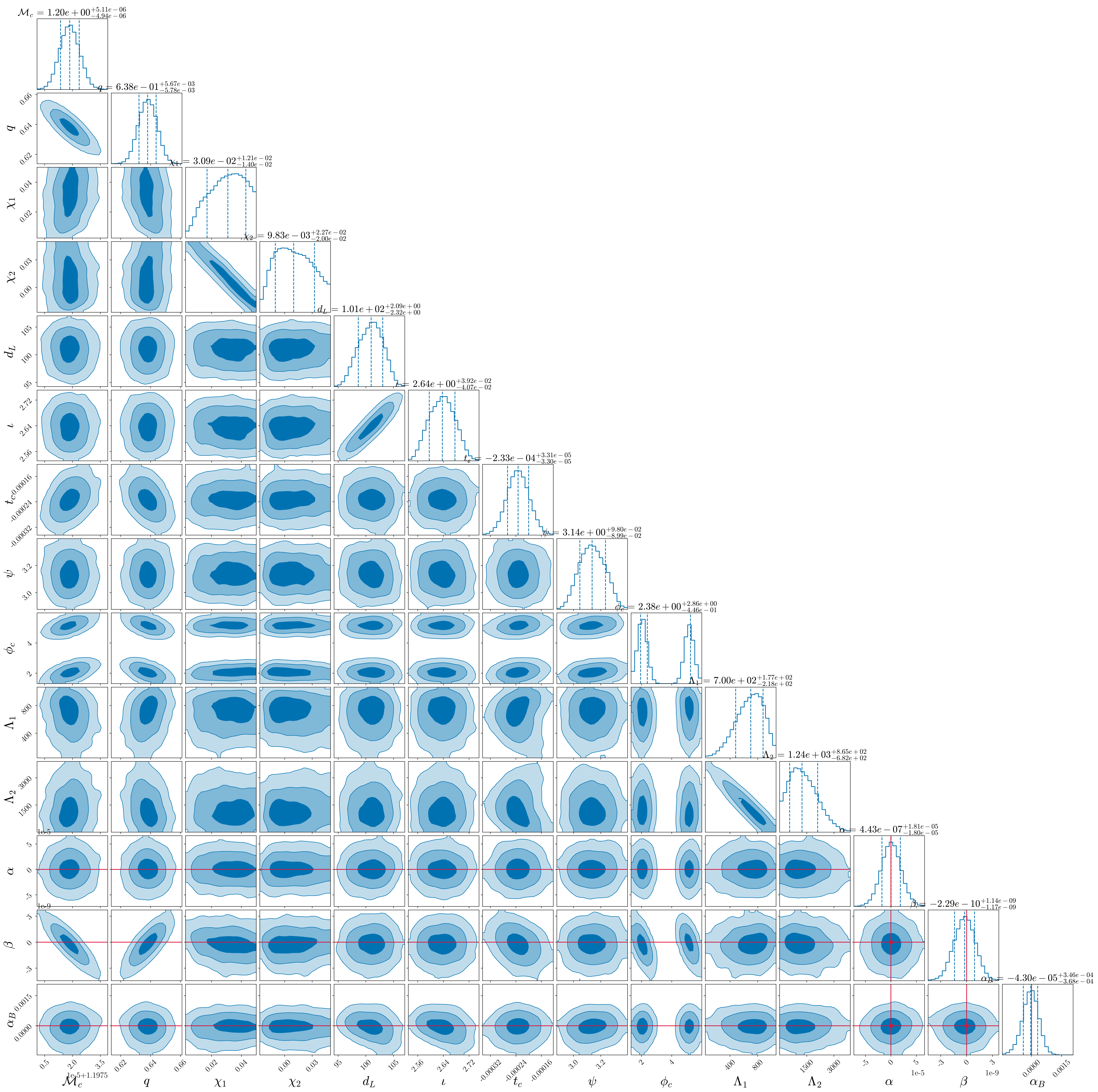
2xCE -- All Parameters (representative BNS)
