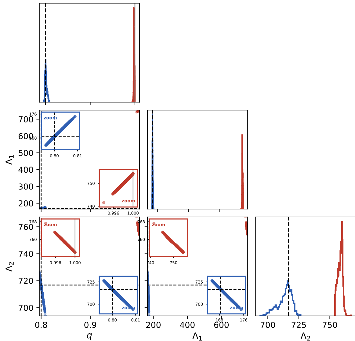
(a) d_L = 42 Mpc (SNR \approx 3355 , anchor)
