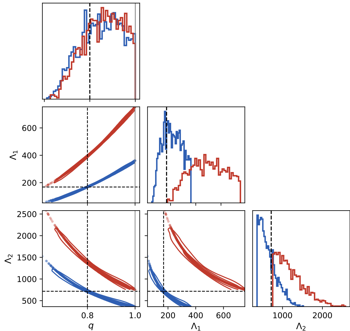
(b) d_L = 9400 Mpc (SNR \approx 15 )
