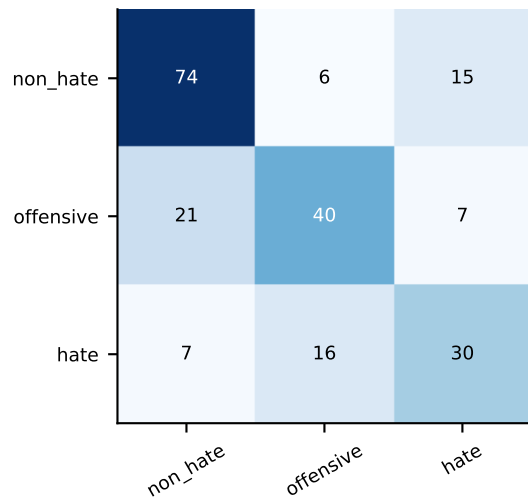
exp1_tfidf_baseline F1=0.510
