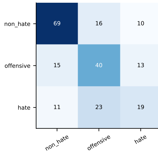
exp8_llm_fewshot F1=0.393
