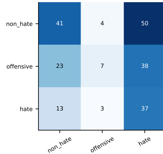
exp7_llm_zeroshot F1=0.354
