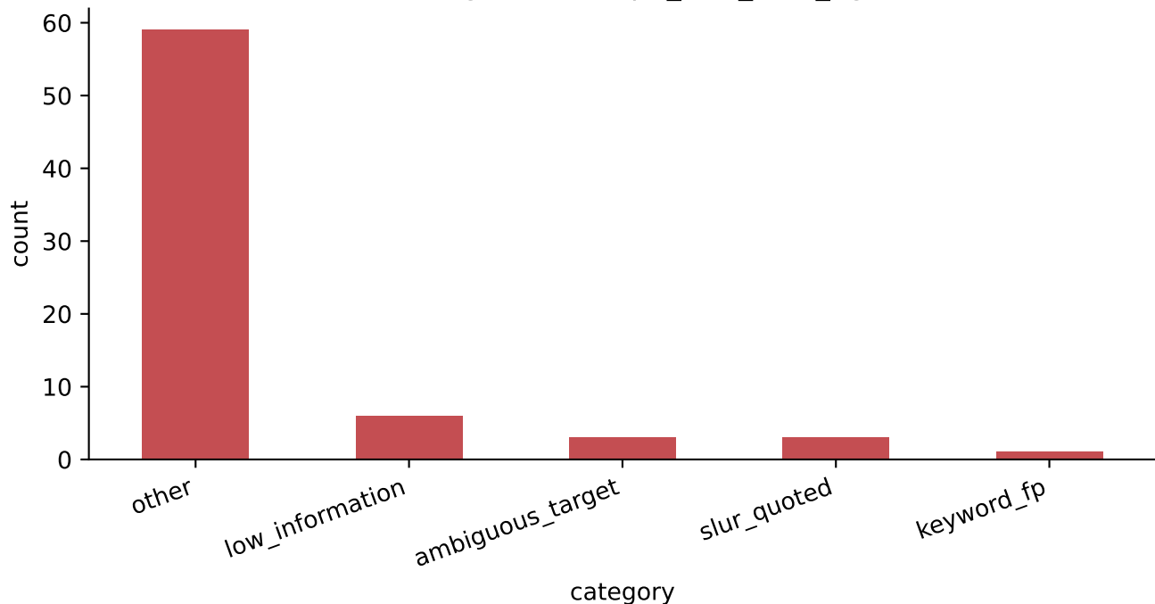
Error categories — exp3_tfidf_char_ngram
