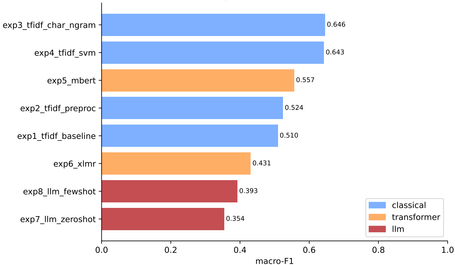
Model comparison — macro-F1 on test set
