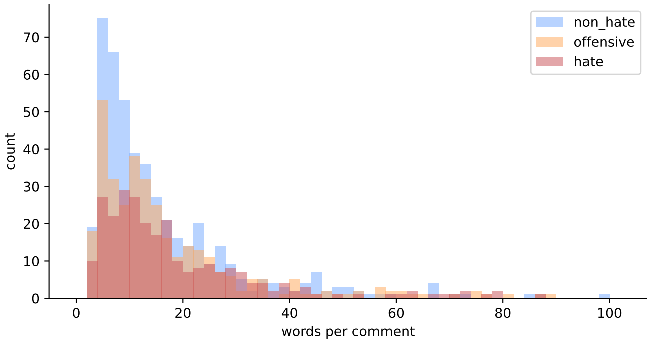
Text length by class
