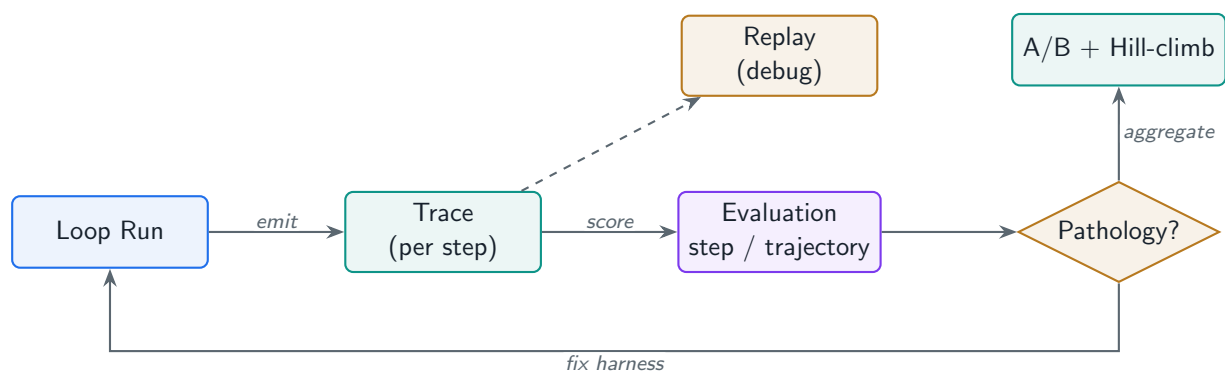
Figure 13.1: Traces flow from runs into per-step, trajectory, run, and fleet evaluation; the aggregate feeds A/B tests and the hill-climbing loop, while replay serves single-run debugging.
