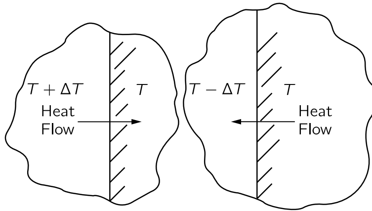
Fig. 44-4. Reversible heat transfer.
