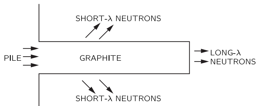
Fig. 38-7. Diffusion of pile neutrons through graphite block.
