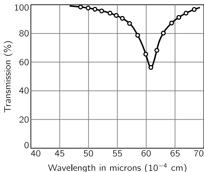
Fig. 23-7. Transmission of infrared radiation through a thin ( 0.17 \mu\text{m} ) sodium chloride film. [After R. B. Barnes, Z. Physik 75 , 723 (1932). Kittel, Introduction to Solid State Physics , Wiley, 1956.]
