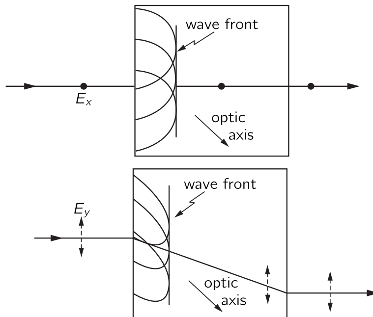
Fig. 33–7. The upper diagram shows the path of the ordinary ray through a doubly refracting crystal.
