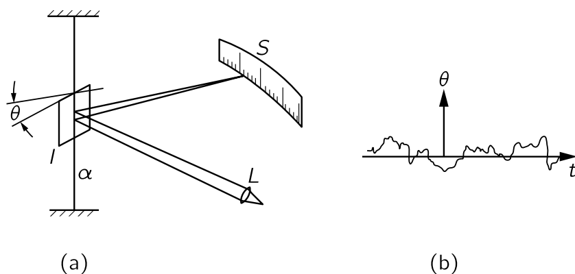
Fig. 41-1. (a) A sensitive light-beam galvanometer. Light from a source L is reflected from a small mirror onto a scale. (b) A schematic record of the reading of the scale as a function of the time.
