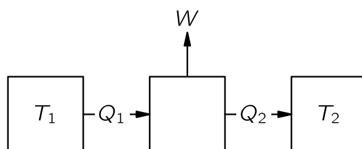
Fig. 44–3. Heat engine.
