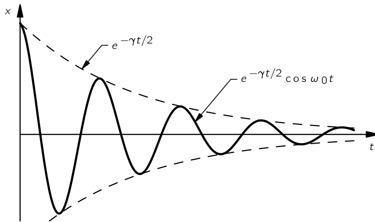
Fig. 24-1. A damped cosine oscillation.
