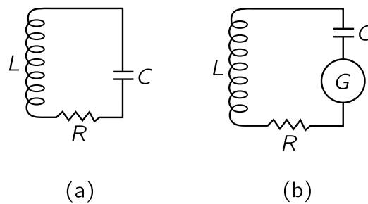
Fig. 41-2. A high- Q resonant circuit. (a) Actual circuit, at temperature T . (b) Artificial circuit, with an ideal (noiseless) resistance and a “noise generator” G .
