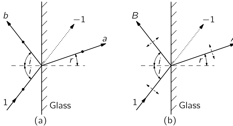
Fig. 33-6. An incident wave of unit amplitude is reflected and refracted at a glass surface. In (a) the incident wave is linearly polarized normal to the plane of the paper. In (b) the incident wave is linearly polarized in the direction shown by the dashed arrows.
