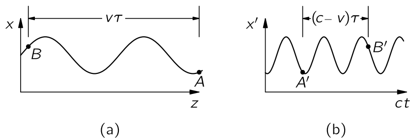
Fig. 34–10. The x - z and x' - t curves of a moving oscillator.
