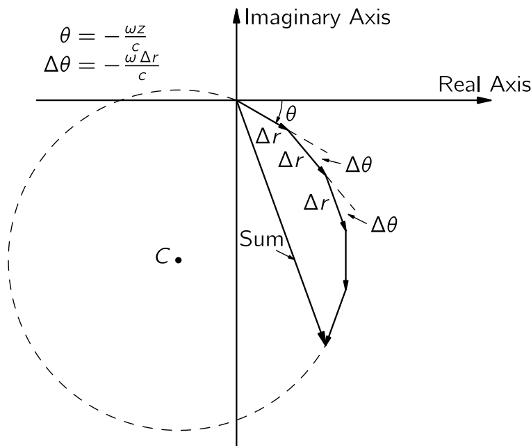
Fig. 30-11. Graphical solution of \int_z^\infty e^{-i\omega r/c} dr .
