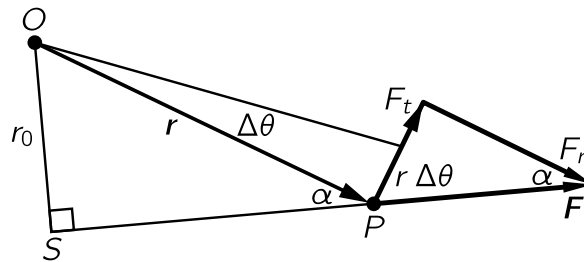
Fig. 18-2. The torque produced by a force.
