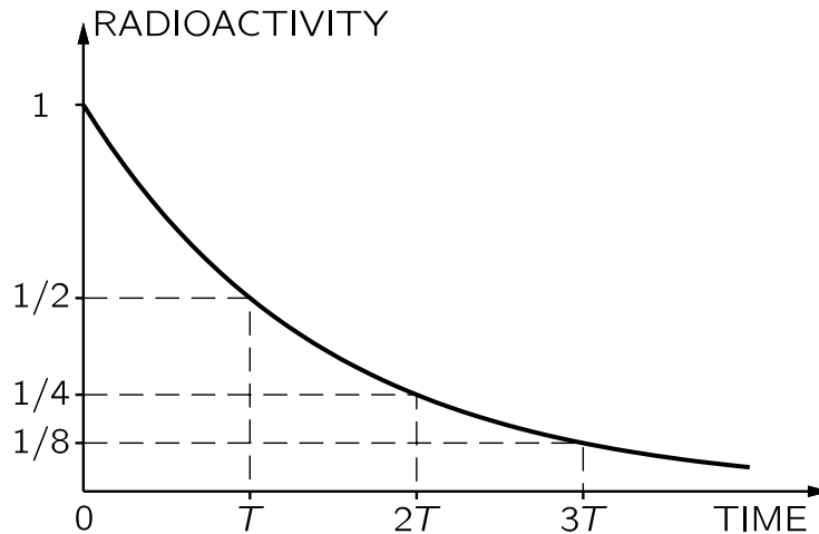
Fig. 5-3. The decrease with time of radioactivity. The activity decreases by one-half in each “half-life,” T .
