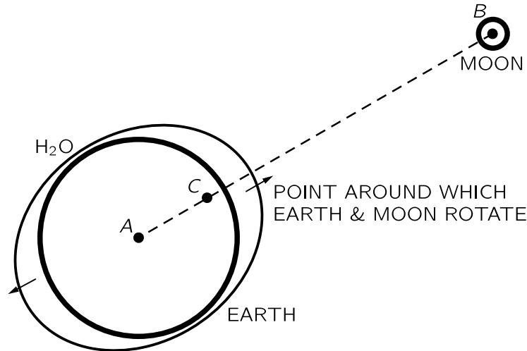
Fig. 7-5. The earth-moon system, with tides.
