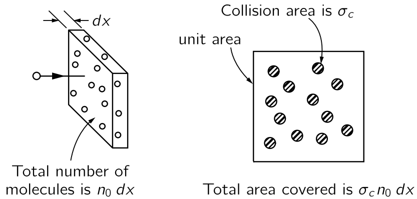
Fig. 43-1. Collision cross section.
