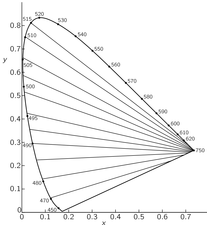
Fig. 35-7. Loci of colors confused by protanopes.
