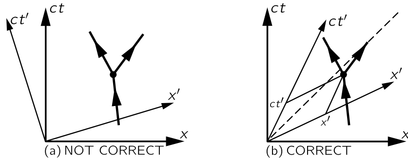
Fig. 17-2. Two views of a disintegrating particle.
