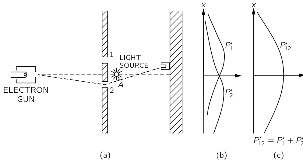
Fig. 37-4. A different electron experiment.
