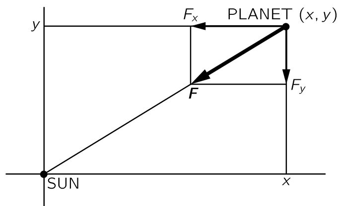
Fig. 9-5. The force of gravity on a planet.
