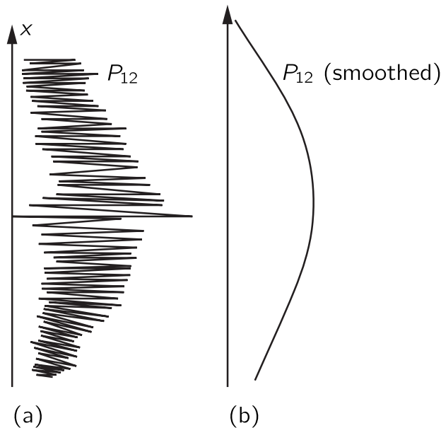
Fig. 37-5. Interference pattern with bullets: (a) actual (schematic), (b) observed.
