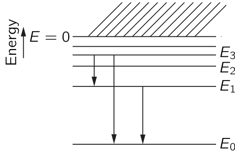
Fig. 38–9. Energy diagram for an atom, showing several possible transitions.
