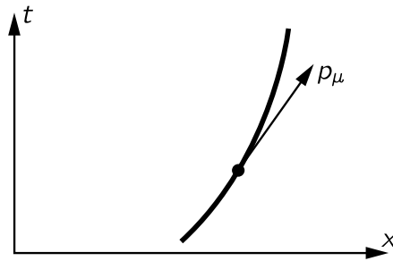
Fig. 17-4. The four-vector momentum of a particle.
