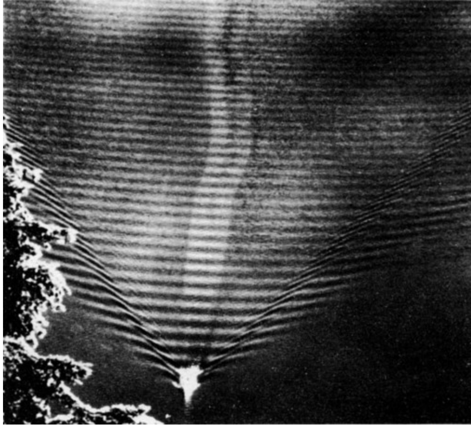
Fig. 51–10. The wake of a boat.
