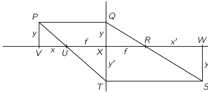
Fig. 27-7. The geometry of imaging by a thin lens.
