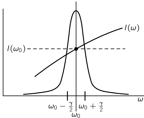
Fig. 41-3. The factors in the integrand (41.10). The peak is the resonance curve 1/[(\omega - \omega_0)^2 + \gamma^2/4] .
