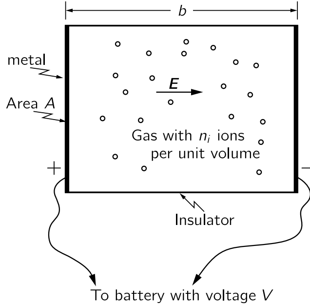
Fig. 43-2. Electric current from an ionized gas.
