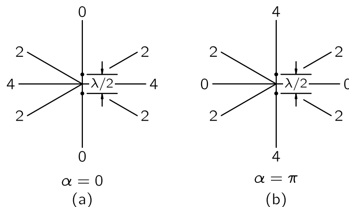
Fig. 29–5. The intensities in various directions from two dipole oscillators one-half wavelength apart. Left: in phase ( \alpha = 0 ). Right: one-half period out of phase ( \alpha = \pi ).
