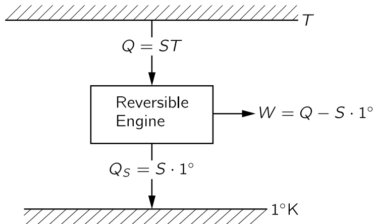
Fig. 44–9. Absolute thermodynamic temperature.
