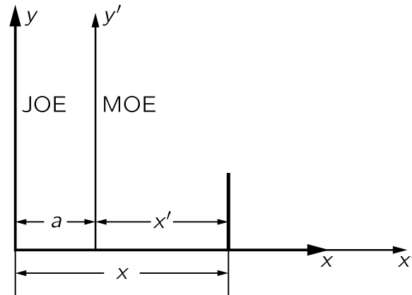
Fig. 11-1. Two parallel coordinate systems.
