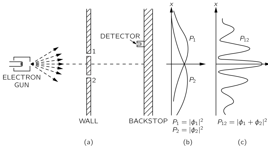
Fig. 37-3. Interference experiment with electrons.
