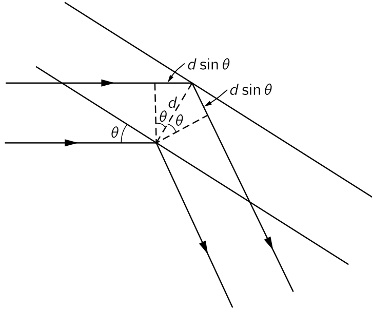
Fig. 38–4. Scattering of waves by crystal planes.
