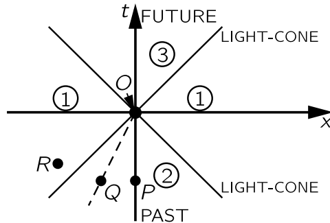
Fig. 17-3. The space-time region surrounding a point at the origin.
