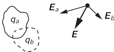
Fig. 25-2. The principle of superposition in electrostatics.
