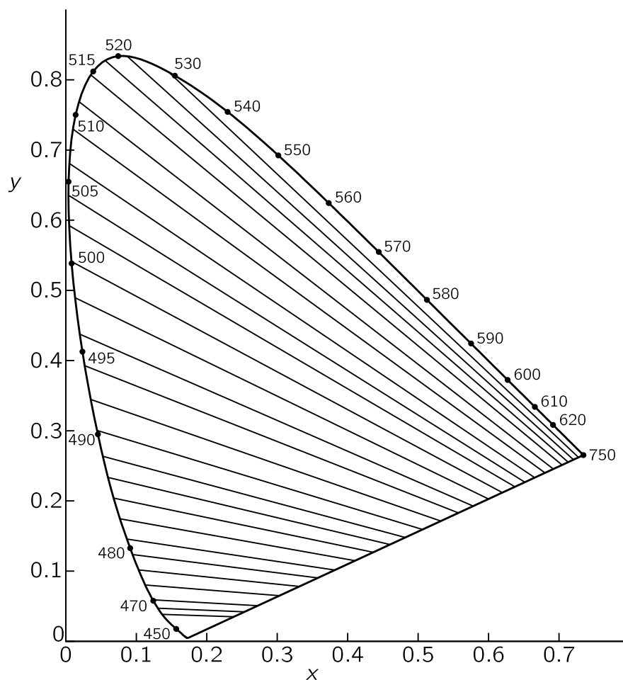
Fig. 35-6. Loci of colors confused by deuteranopes.
