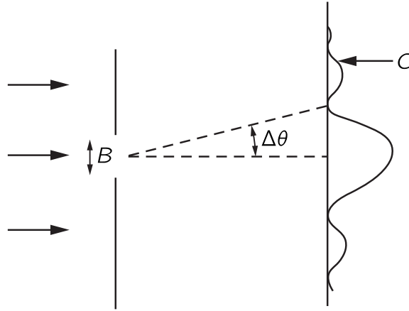
Fig. 38-2. Diffraction of particles passing through a slit.
