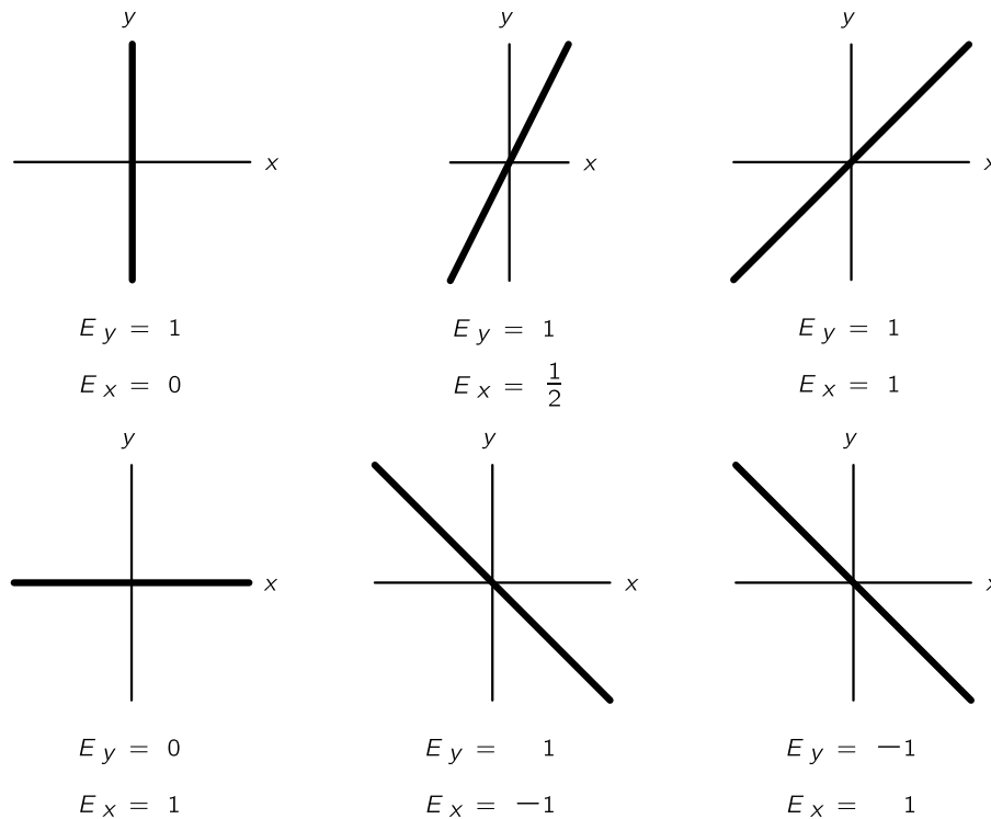
Fig. 33-1. Superposition of x -vibrations and y -vibrations in phase.
