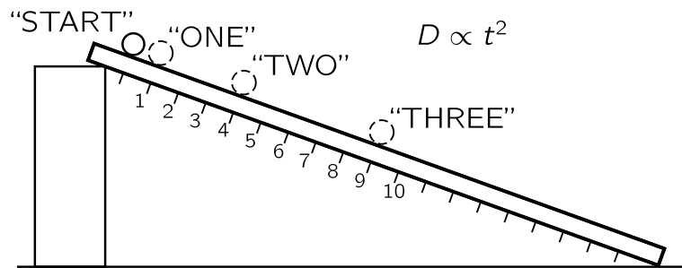
Fig. 5-1. A ball rolls down an inclined track.
