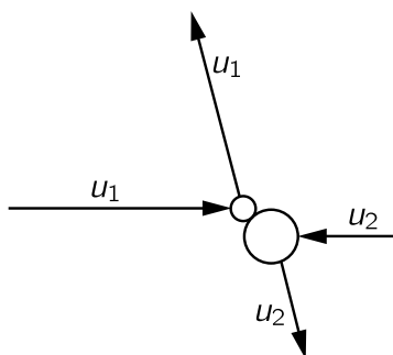
Fig. 39–3. A collision between unequal atoms, viewed in the CM system. u_1 = |\mathbf{v}_1 - \mathbf{v}_{\text{CM}}| ,
