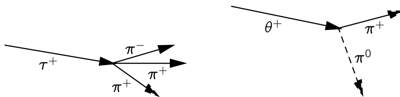
Fig. 52–5. A schematic diagram of the disintegration of a \tau^+ and a \theta^+ particle.
