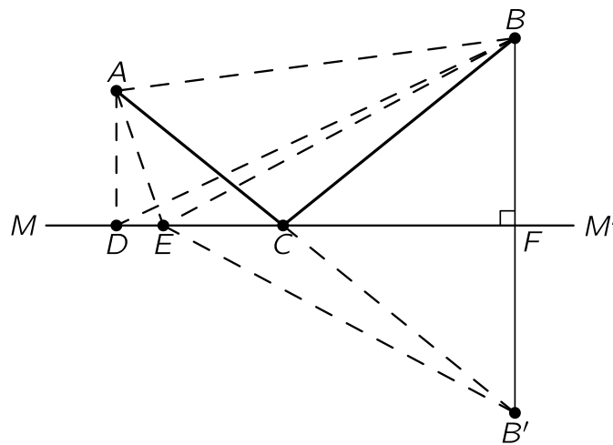
Fig. 26-3. Illustration of the principle of least time.
