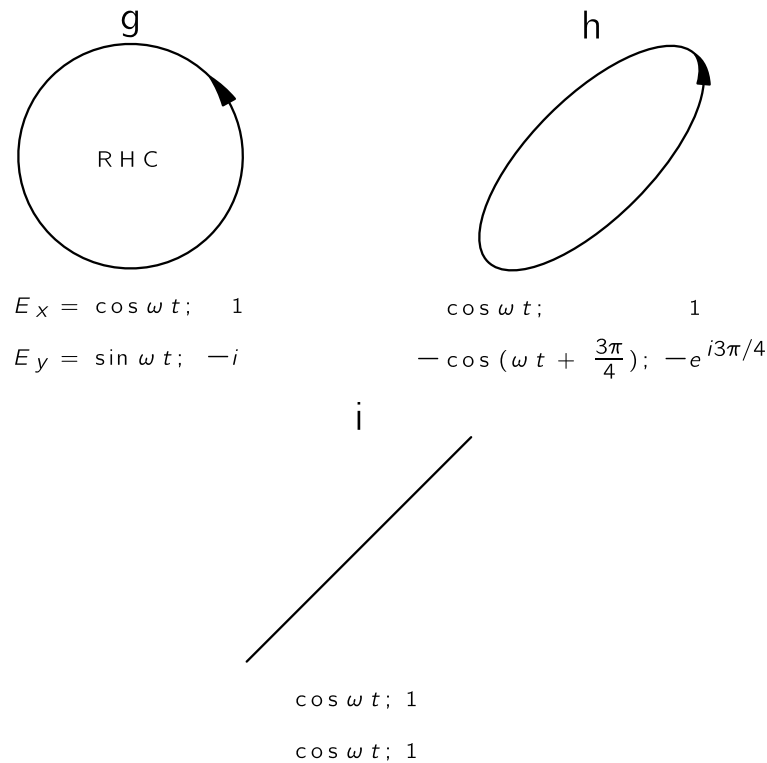
Fig. 33-2. Superposition of x-vibrations and y-vibrations with equal amplitudes but various relative phases. The components E_x and E_y are expressed in both real and complex notations.
