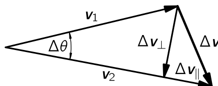
Fig. 11-8. Diagram for calculating the acceleration.
