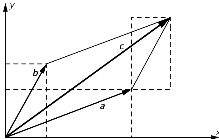
Fig. 11-4. The addition of vectors.
