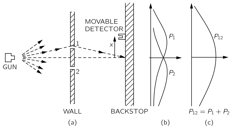
Fig. 37-1. Interference experiment with bullets.
