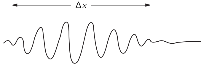
Fig. 38-1. A wave packet of length \Delta x .
