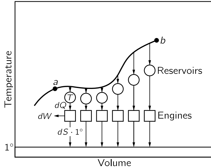
Fig. 44–10. Change in entropy during a reversible transformation.
