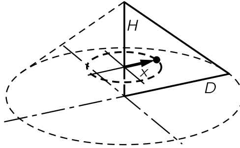
Fig. 19–2. A right triangle and a right circular cone generated by rotating the triangle.
