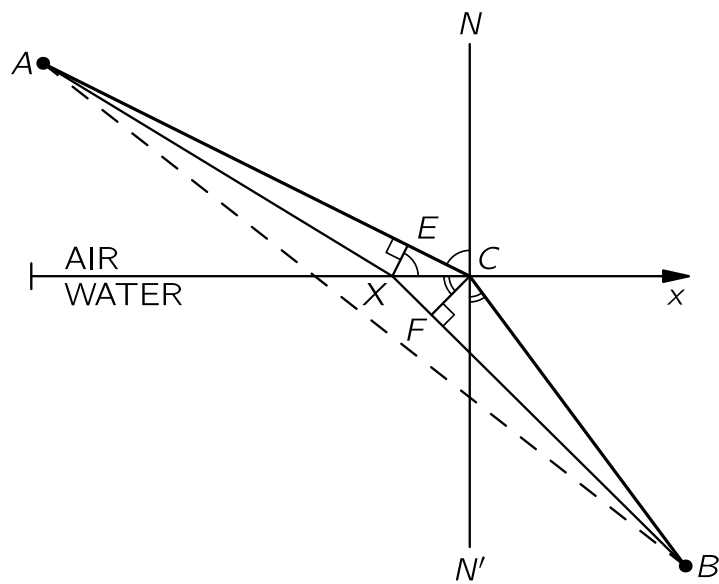
Fig. 26-4. Illustration of Fermat's principle for refraction.
