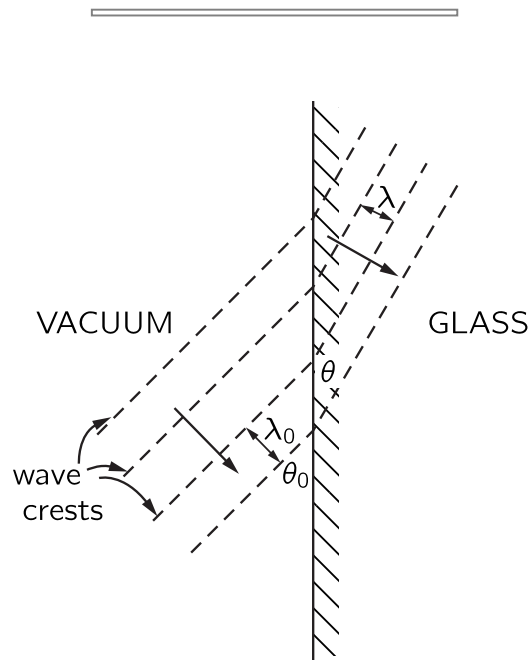
Fig. 31-2. Relation between refraction and velocity change.
