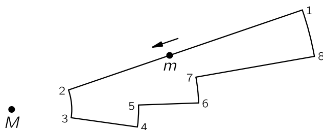
Fig. 13–3. A closed path in a gravitational field.
