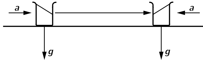
Fig. 12-4. Illustration of a pseudo force.
