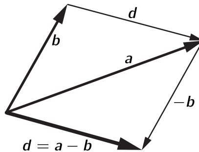
Fig. 11-5. The subtraction of vectors.
