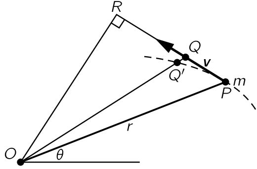
Fig. 18-3. A particle moves about an axis O .
