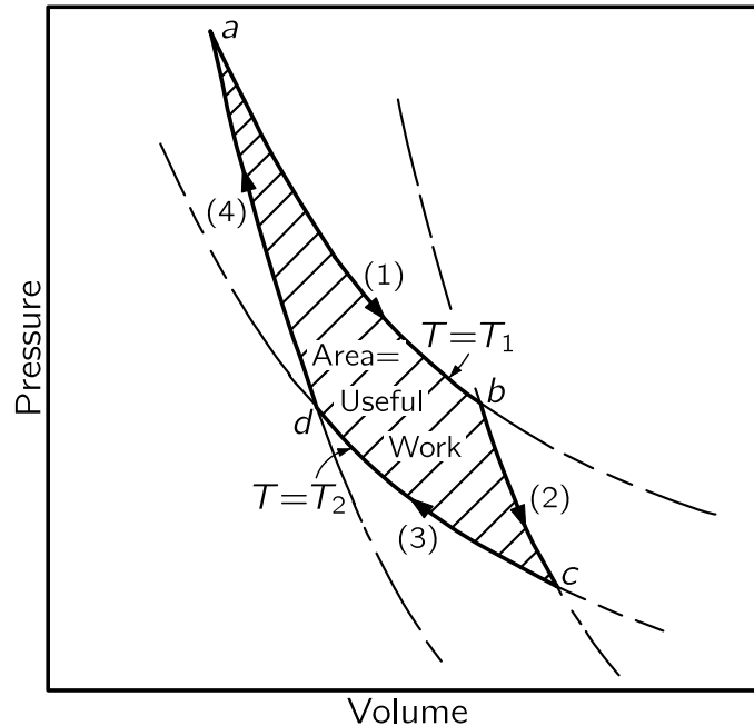
Fig. 44-6. The Carnot cycle.
