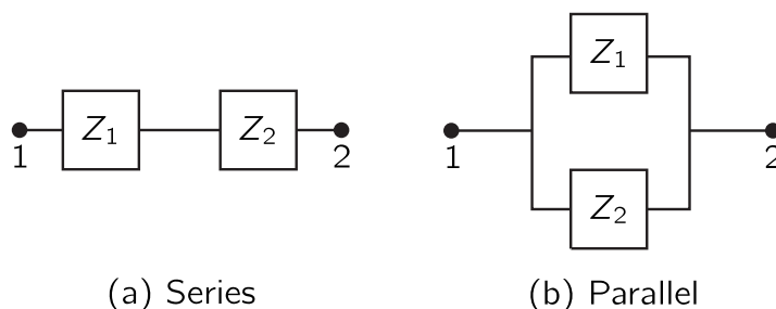
Fig. 25–6. Two impedances, connected in series and in parallel.
