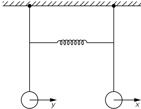
Fig. 49-5. Two coupled pendulums.
