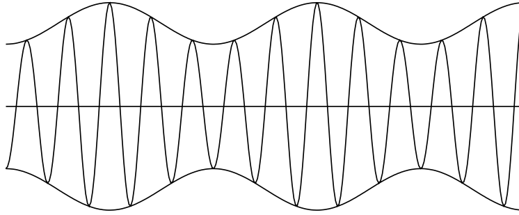
Fig. 48–4. A modulated carrier wave. In this schematic sketch, \omega_c / \omega_m = 5 . In an actual radiowave,
