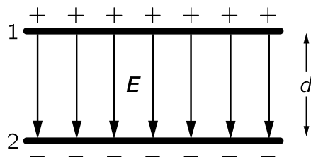
Fig. 14–5. Field between parallel plates.
