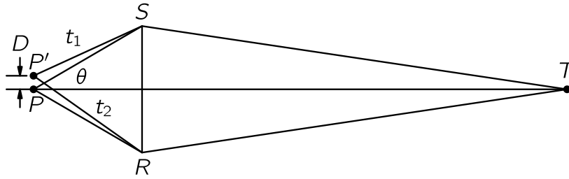
Fig. 27-9. The resolving power of an optical system.
