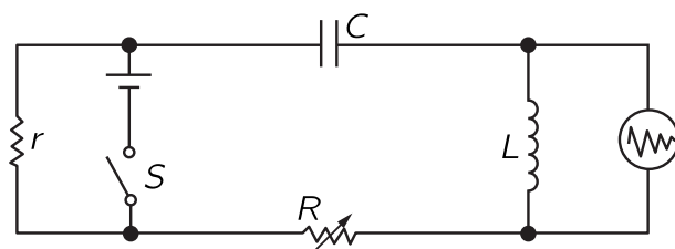
Fig. 24–2. An electrical circuit for demonstrating transients.
