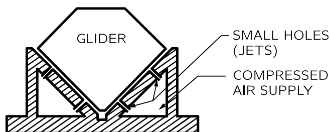
Fig. 10-1. End view of linear air trough.
