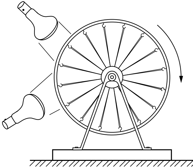
Fig. 44-2. The rubber band heat engine.
