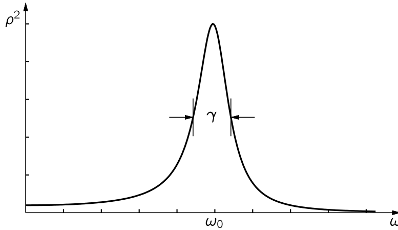
Fig. 23-2. Plot of \rho^2 versus \omega .
