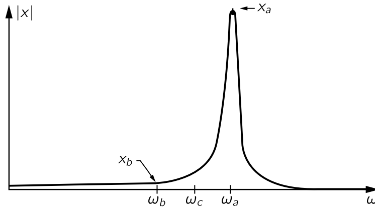
Fig. 25–3. A sharply tuned resonance curve.
