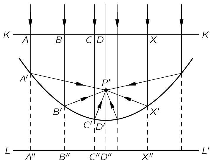
Fig. 26-12. A paraboloidal mirror.
