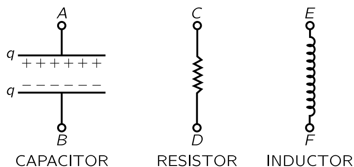
Fig. 23-4. The three passive circuit elements.
