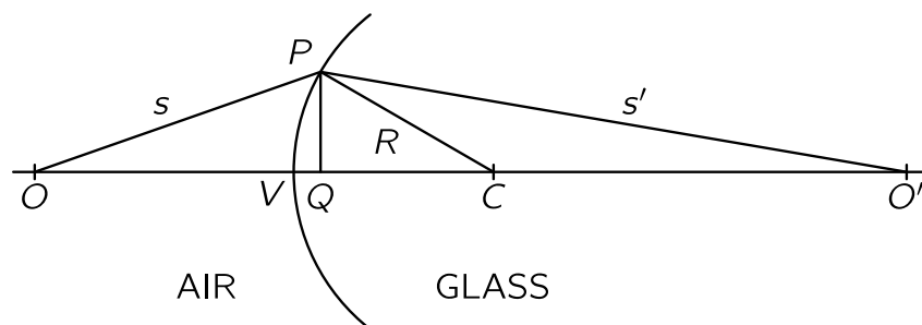
Fig. 27-2. Focusing by a single refracting surface.
