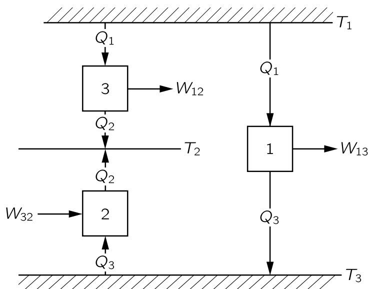
Fig. 44–8. Engines 1 and 2 together are equivalent to engine 3.
