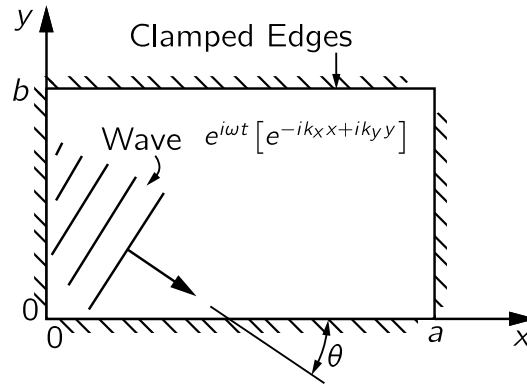
Fig. 49-4. Vibrating rectangular plate.
