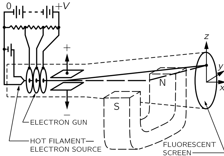
Fig. 12-3. An electron-beam tube.
