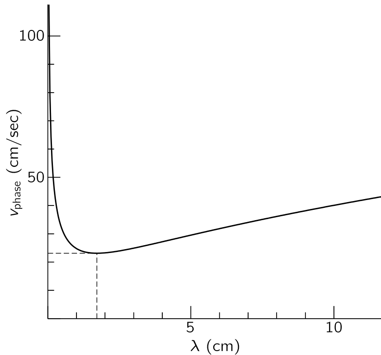
Fig. 51-11. Phase velocity vs. wavelength for water.
