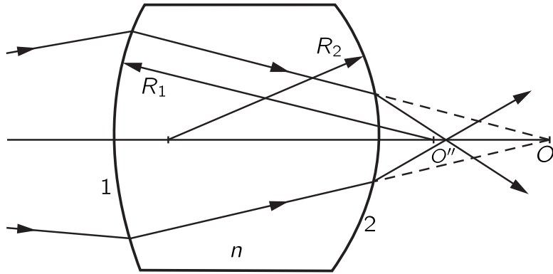
Fig. 27-5. Image formation by a two-surface lens.
