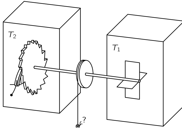
Fig. 46-1. The ratchet and pawl machine.
