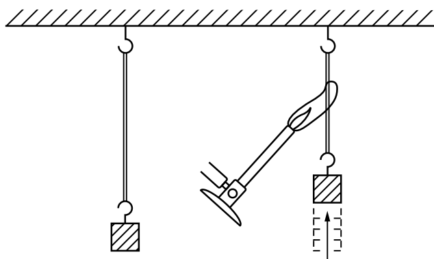
Fig. 44-1. The heated rubber band.
