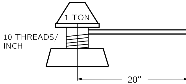
Fig. 4-5. A screw jack.
