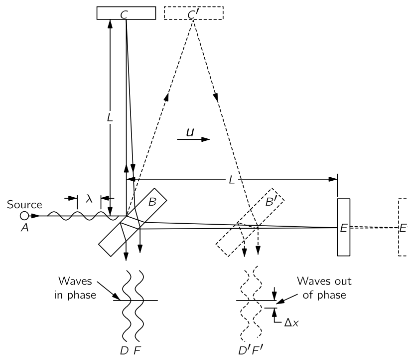
Fig. 15–2. Schematic diagram of the Michelson-Morley experiment.
