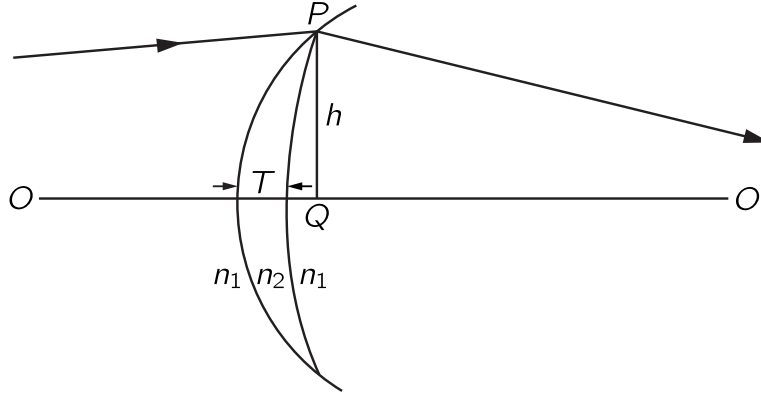
Fig. 27-6. A thin lens with two positive radii.
