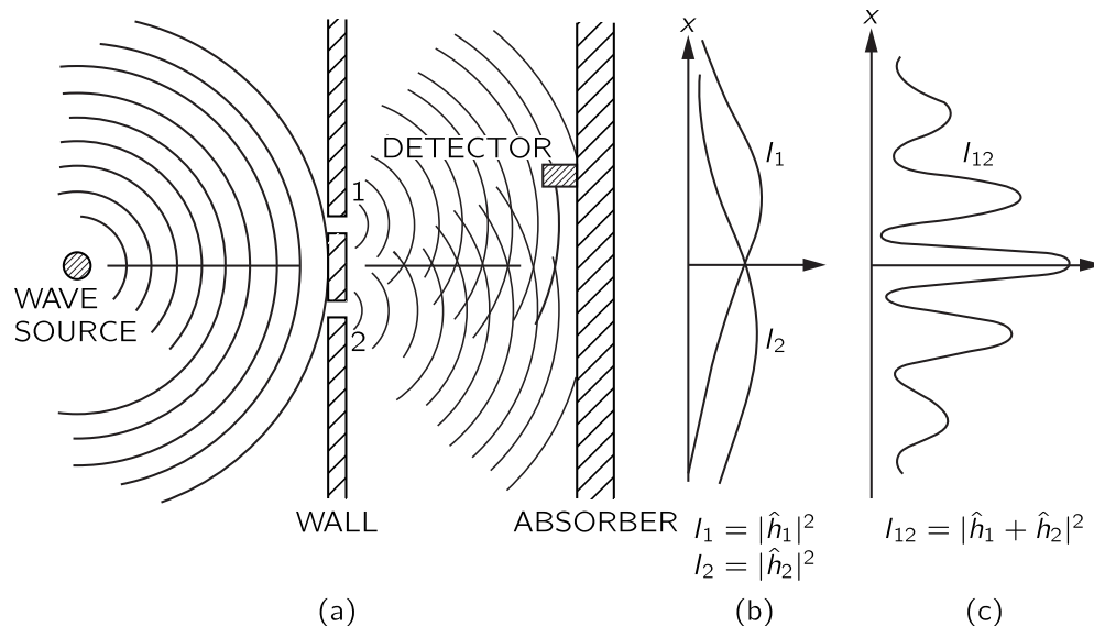
Fig. 37-2. Interference experiment with water waves.
