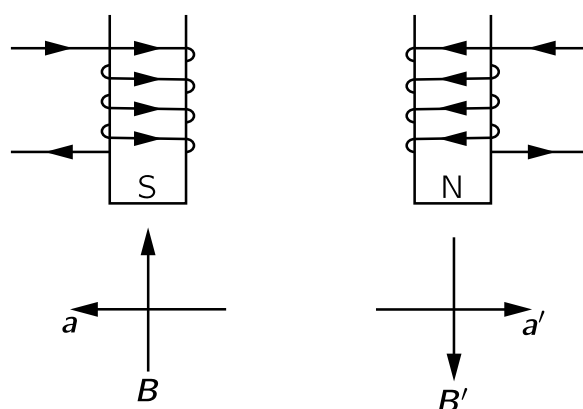
Fig. 52-4. A magnet and its mirror image.
