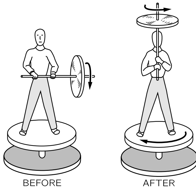
Fig. 20–1. Before : axis is horizontal; moment about vertical axis = 0. After : axis is vertical; momentum about vertical axis is still zero; man and chair spin in direction opposite to spin of the wheel.
