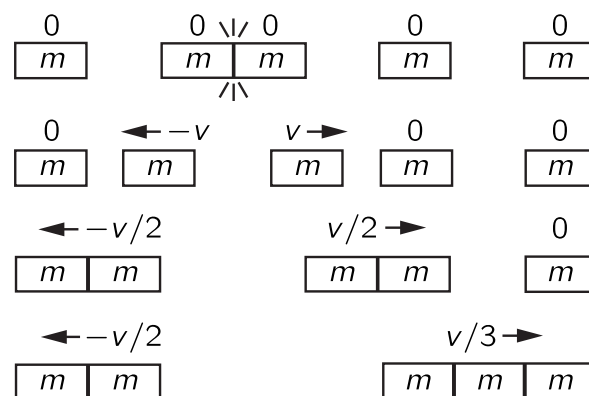
Fig. 10-8. Action and reaction between 2m and 3m .
