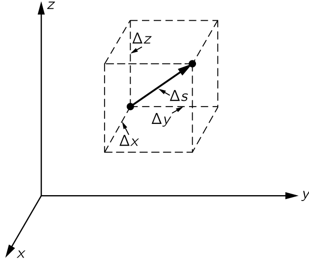
Fig. 9-1. A small displacement of an object.
