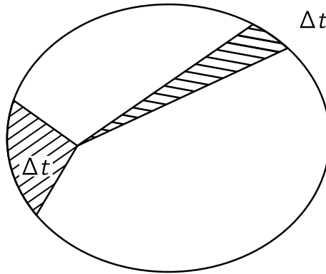
Fig. 7-2. Kepler's law of areas.
