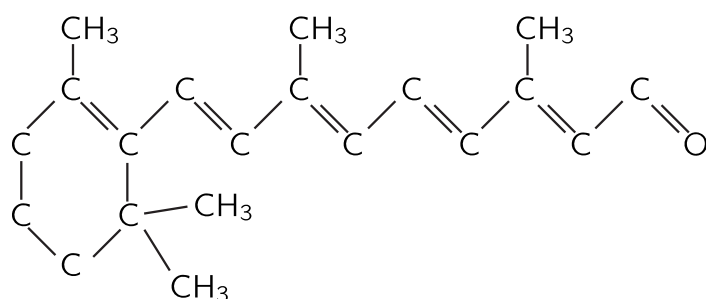
Fig. 36-6. The structure of retinene.
