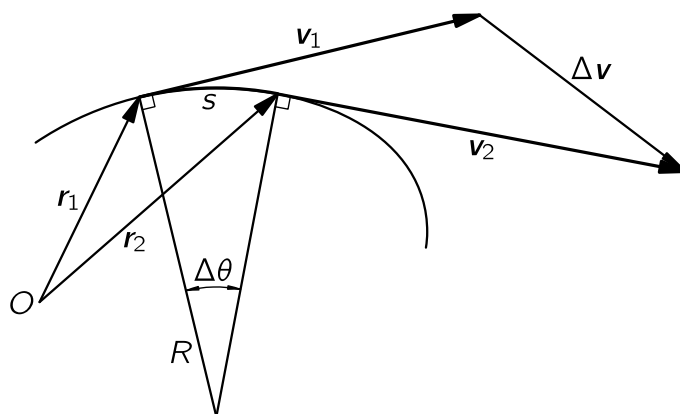
Fig. 11-7. A curved trajectory.
