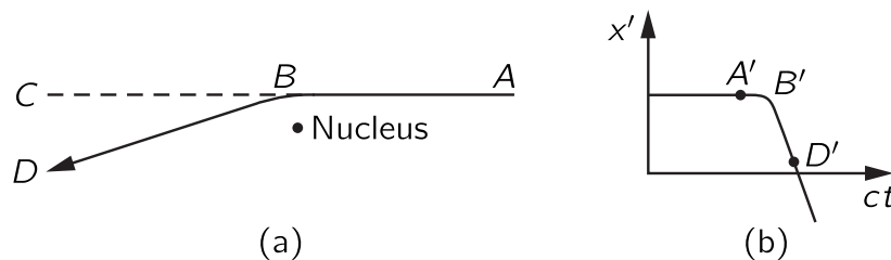
Fig. 34–9. A fast electron passing near a nucleus radiates energy in the direction of its motion.
