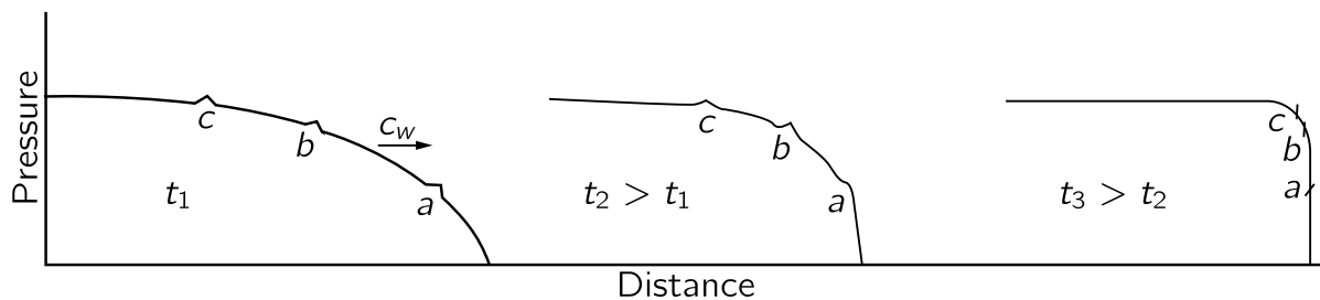
Fig. 51–3. Wavefront “snapshots” at successive instants in time.
