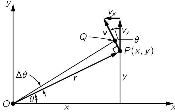
Fig. 18-1. Kinematics of two-dimensional rotation.
