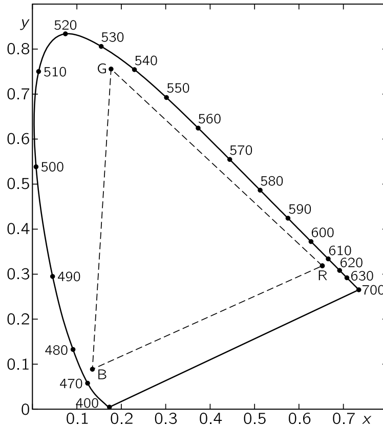
Fig. 35-4. The standard chromaticity diagram.
