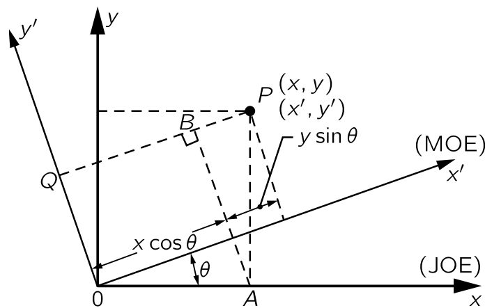
Fig. 11-2. Two coordinate systems having different angular orientations.
