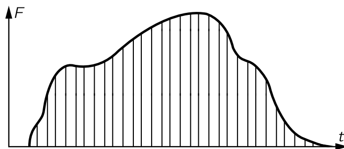
Fig. 25-4. A complicated force may be treated as a succession of sharp impulses.
