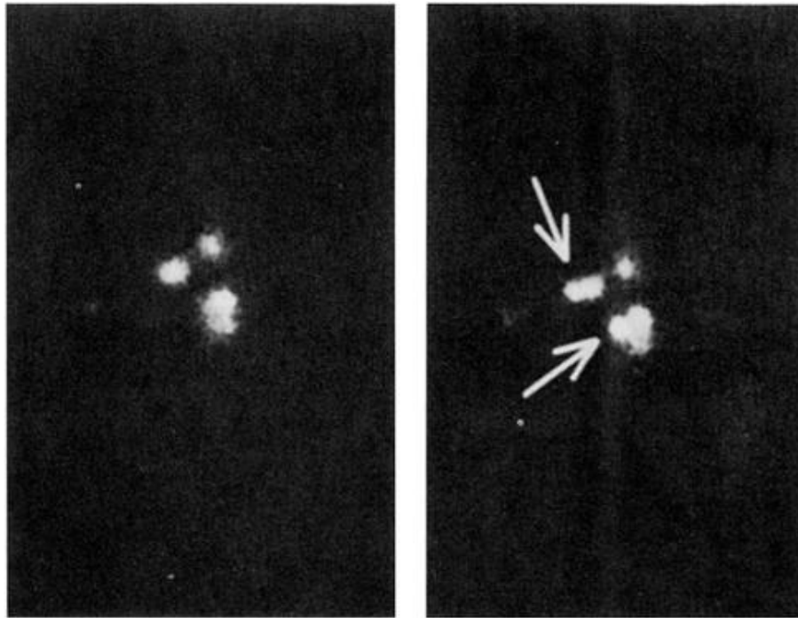
Fig. 7-12. The formation of new stars?
