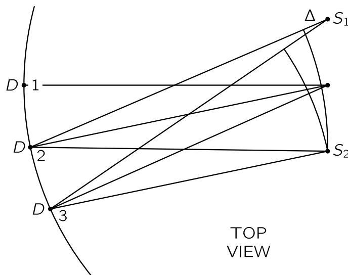
Fig. 28–3. Illustration of interference of sources.
