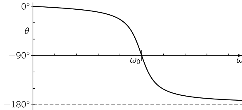
Fig. 23-3. Plot of \theta versus \omega .
