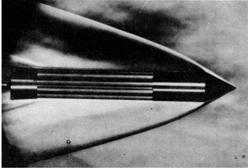
Fig. 51-2. A shock wave induced in a gas by a projectile moving faster than sound.
