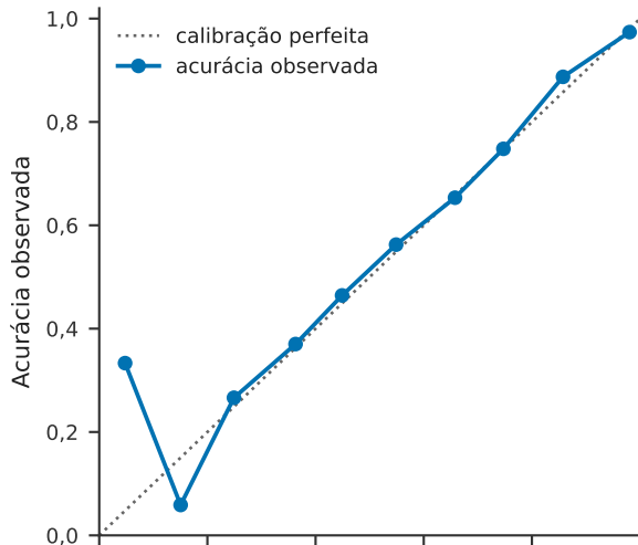
Extra Trees
