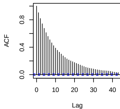
ACF: z_bmi
