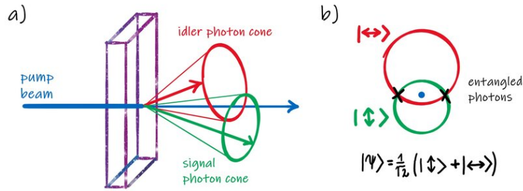
FIGURE 03.19D.2: Diagram of Spontaneous Parametric Down Conversion (SPDC) process. Source: Applications of single-photon technology - Scientific Figure on ResearchGate. Available from: https://www.researchgate.net/figure/The-SPDC-cones-a-Type-II-process-b-Polarization-entangled-photon-pair_fig10_360782305 [accessed 19 Mar 2025].
