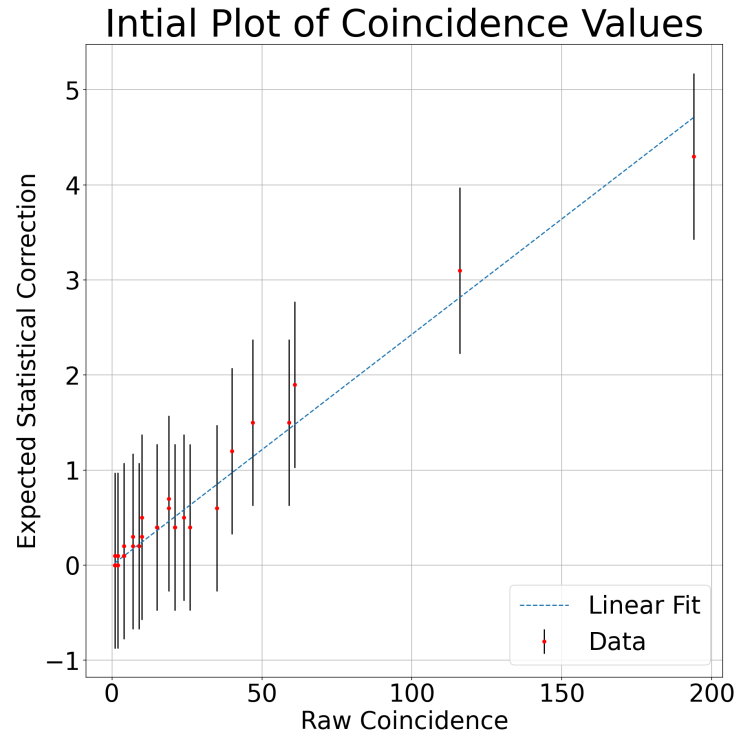
FIGURE 03.11A.3: Initial fit of coincidence values and expected statistical correction. Slope found is given by \tau = 0.0243 \pm 0.0006 with a \chi^2_{\text{red}} = 0.03 .
