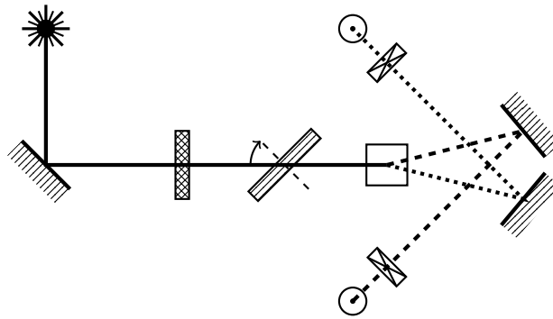
FIGURE 03.19E.3: Experimental setup (405 nm).
