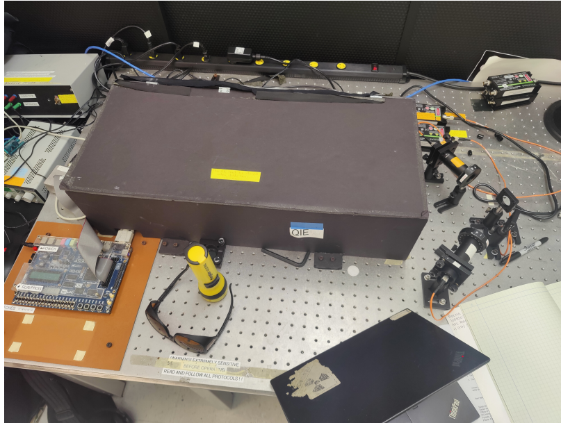
FIGURE 03.11A.1: Initial experimental setup prior to any changes. All components seem to be in place. Noticed no caps on extra APD detectors.
