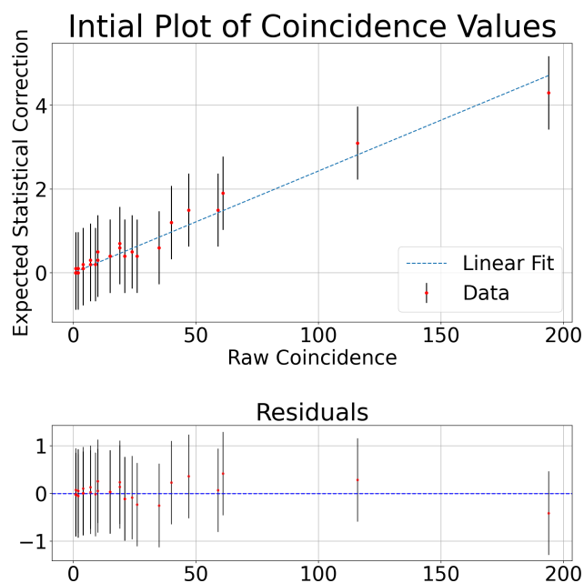
FIGURE 03.14A.1: Same fit of data as in Fig. 03.11A.3 but with residuals.
