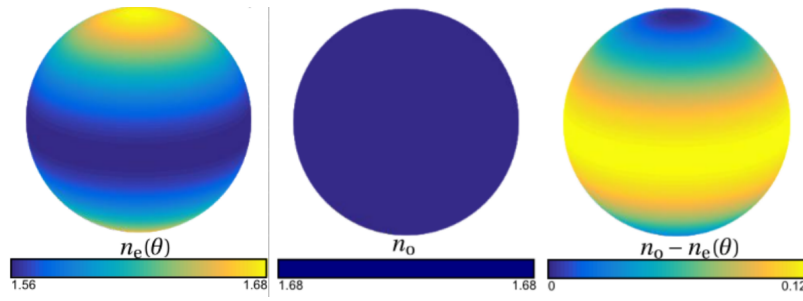
FIGURE 03.22A.1 : The extraordinary and ordinary refractive indices (and their difference) as a function of direction for beta barium borate (BBO) at \lambda = 500 nm ( n_o = 1.68 and n_e = 1.56 ) [5].
