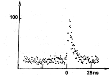
FIGURE 03.30B.1: Illustration between delay time and coincidence rate [7] known as the Time Delay Spectrum . The flat background corresponds with accidental coincidences between uncorrelated photons emitted by different atoms and scales with the square, N^2 , of the cascade rate. The peak, whose area scales with N , corresponds with the correlated photons and gives the coincidences to be measured.
