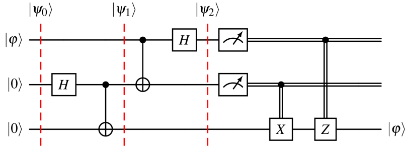
FIGURE 04.03C.1: Quantum teleportation circuit as described (with modification) by Nielson and Chuang [2]. The first Hadamard ( \hat{H} ) and CNOT gates describe the creation of a Bell state. Figure and caption from [3].
