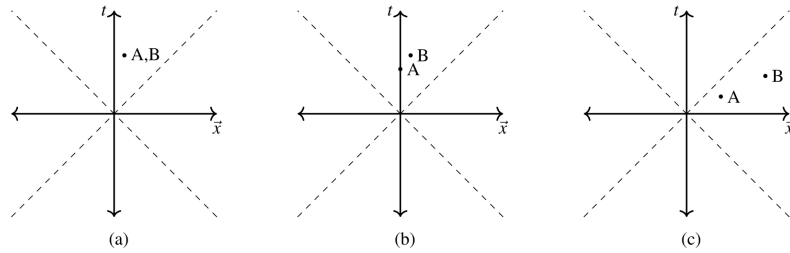
FIGURE 04.03B.1: (a) Two events/interactions at the same space-time location are local. (b) Two time-like events separated by a distance preserve Einstein's locality condition. (c) Two space-like separated events are nonlocal. Figure and caption from [3].
