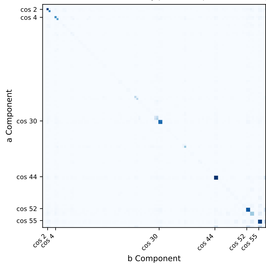
Fourier Coefficients of h_4 (Division (Generator: 3))
