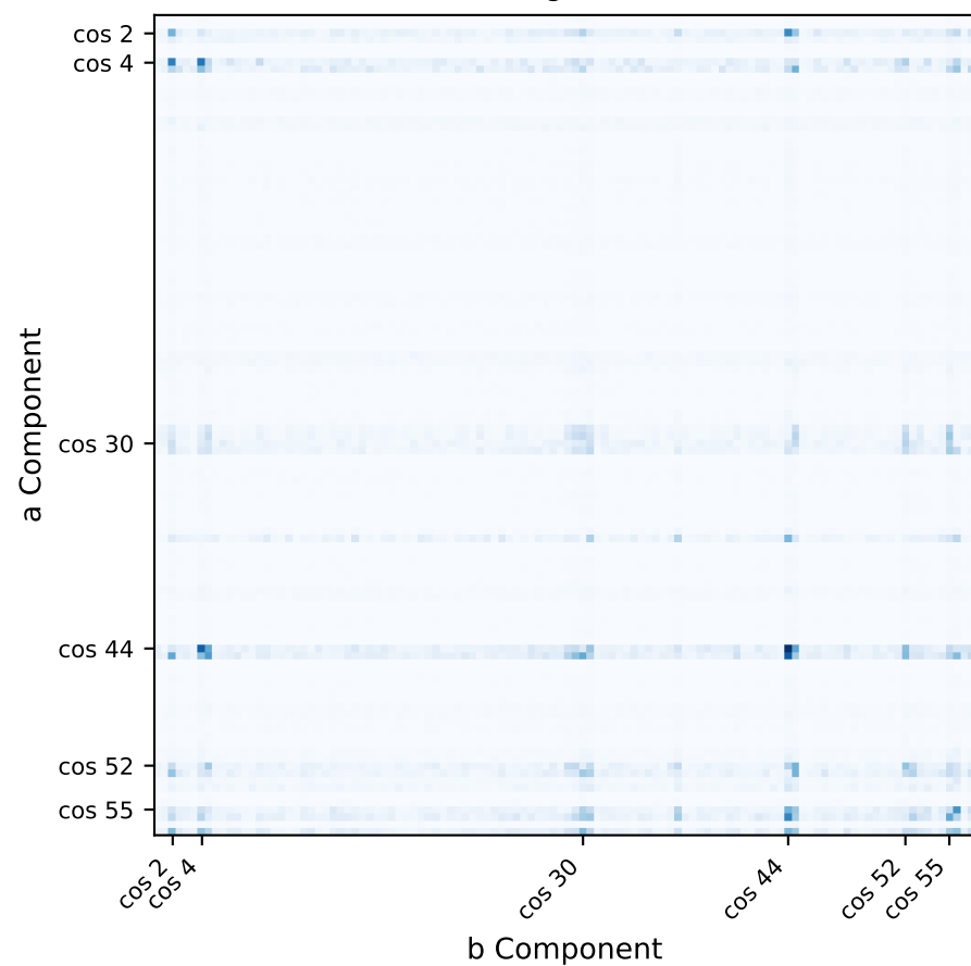
Fourier Coefficients of h_3 (Division (Generator: 3))
