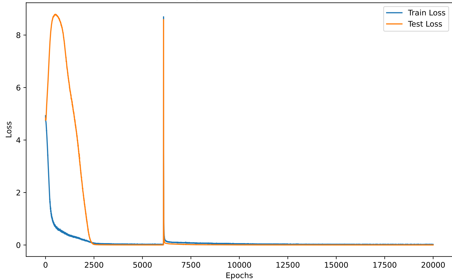
Training and Test Loss Over Time
