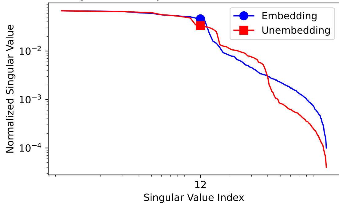
Singular Value Spectrum for Modular Division
