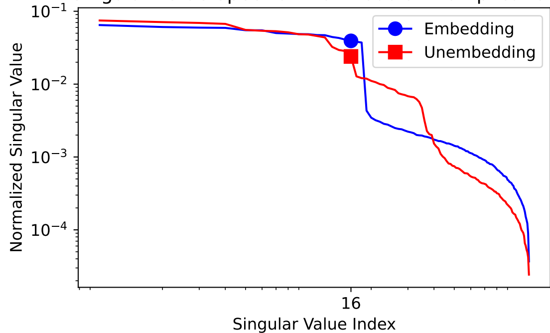
Singular Value Spectrum for Modular Multiplication
