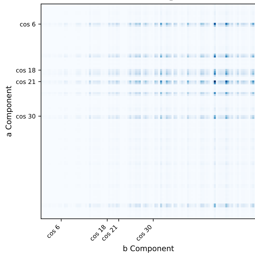
Fourier Coefficients of h_4 (Subtraction)
