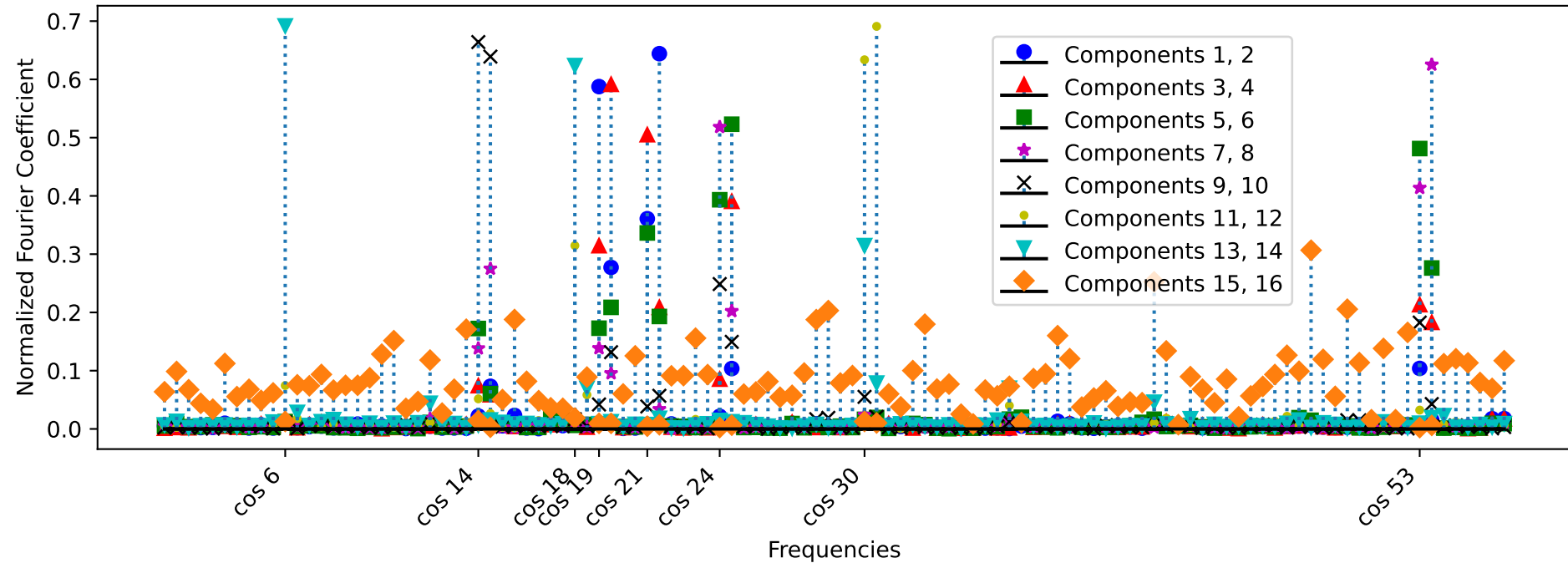
Fourier Coefficients of Components of W_{fc} (Subtraction)
