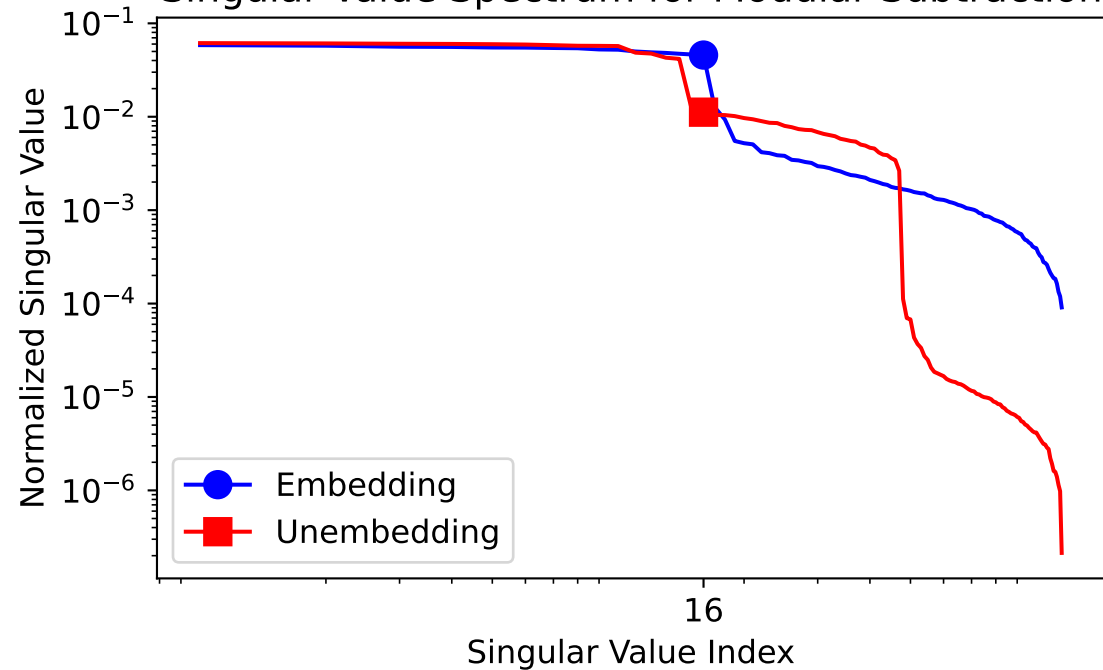
Singular Value Spectrum for Modular Subtraction
