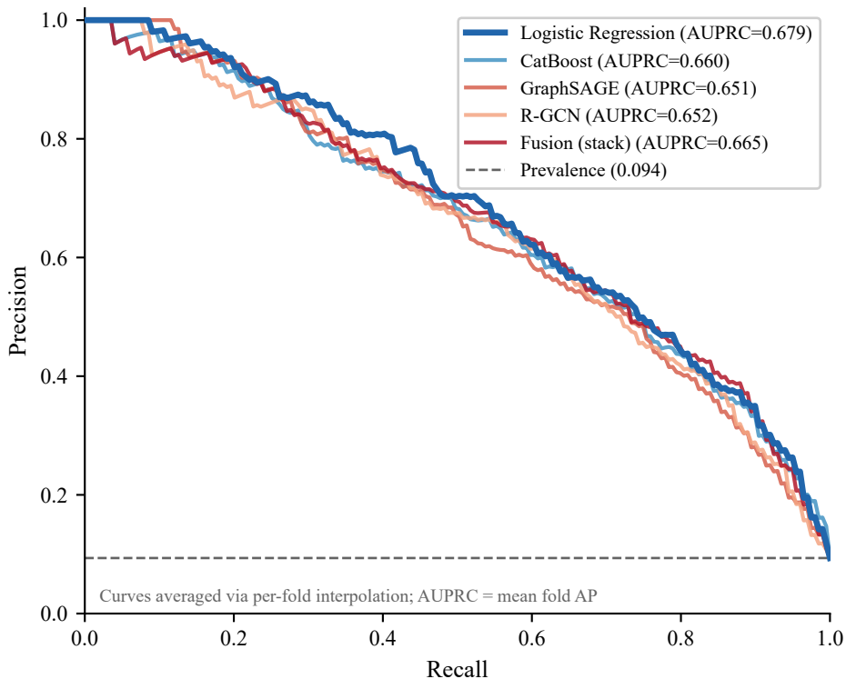
Precision–Recall Curves (mean across 5 folds)
