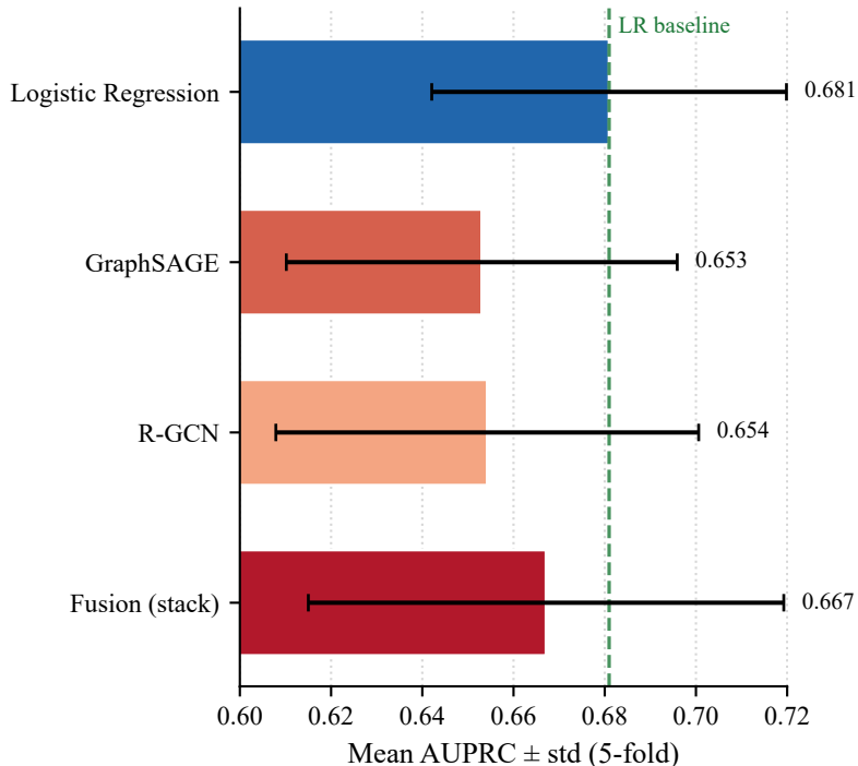
(a) Feature vs Graph Methods
