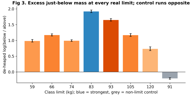
Fig. 3. H2: excess just-below mass at every real limit; control runs opposite
