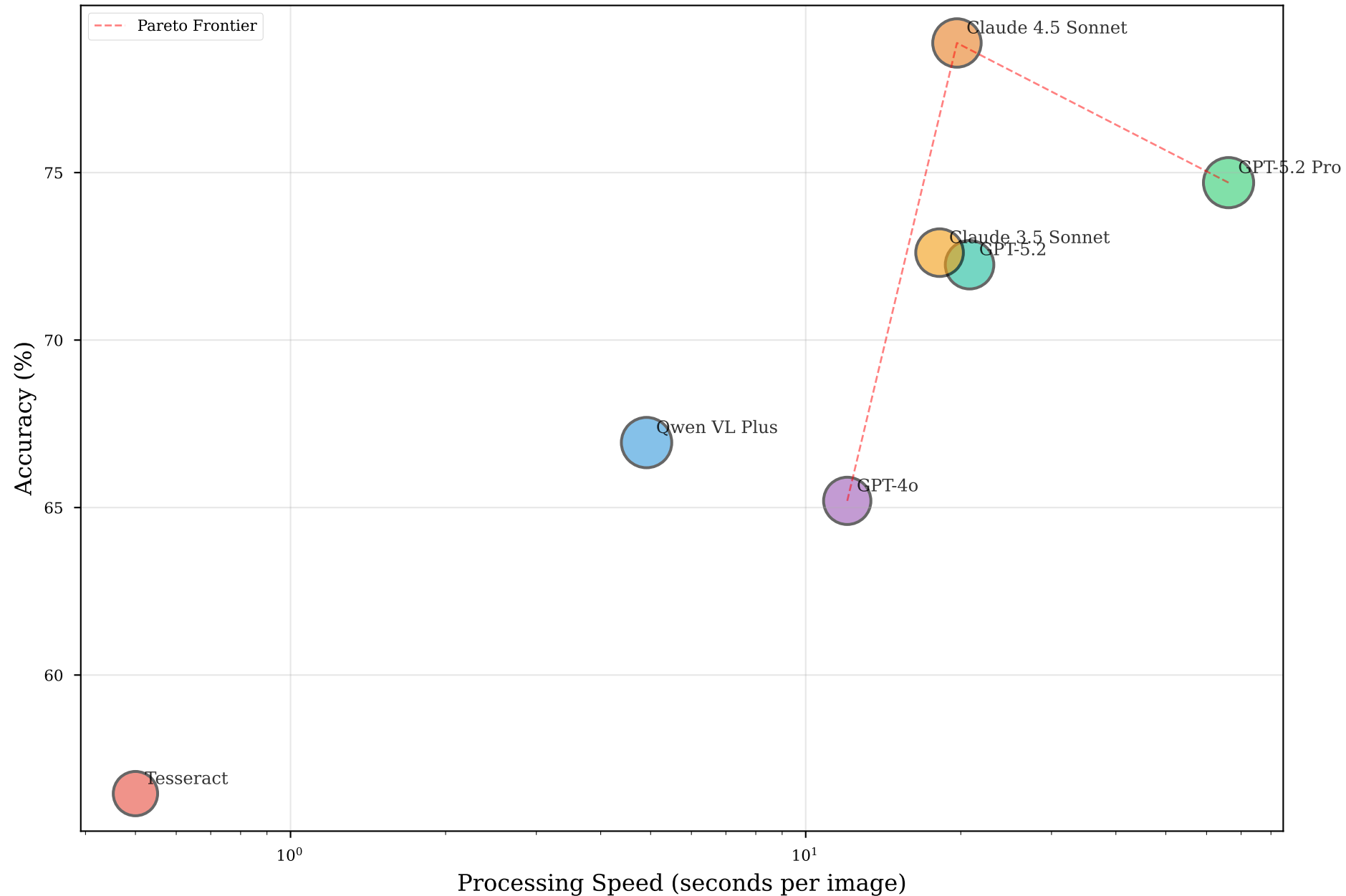
Speed-Accuracy Trade-off (bubble size = F1 score)
