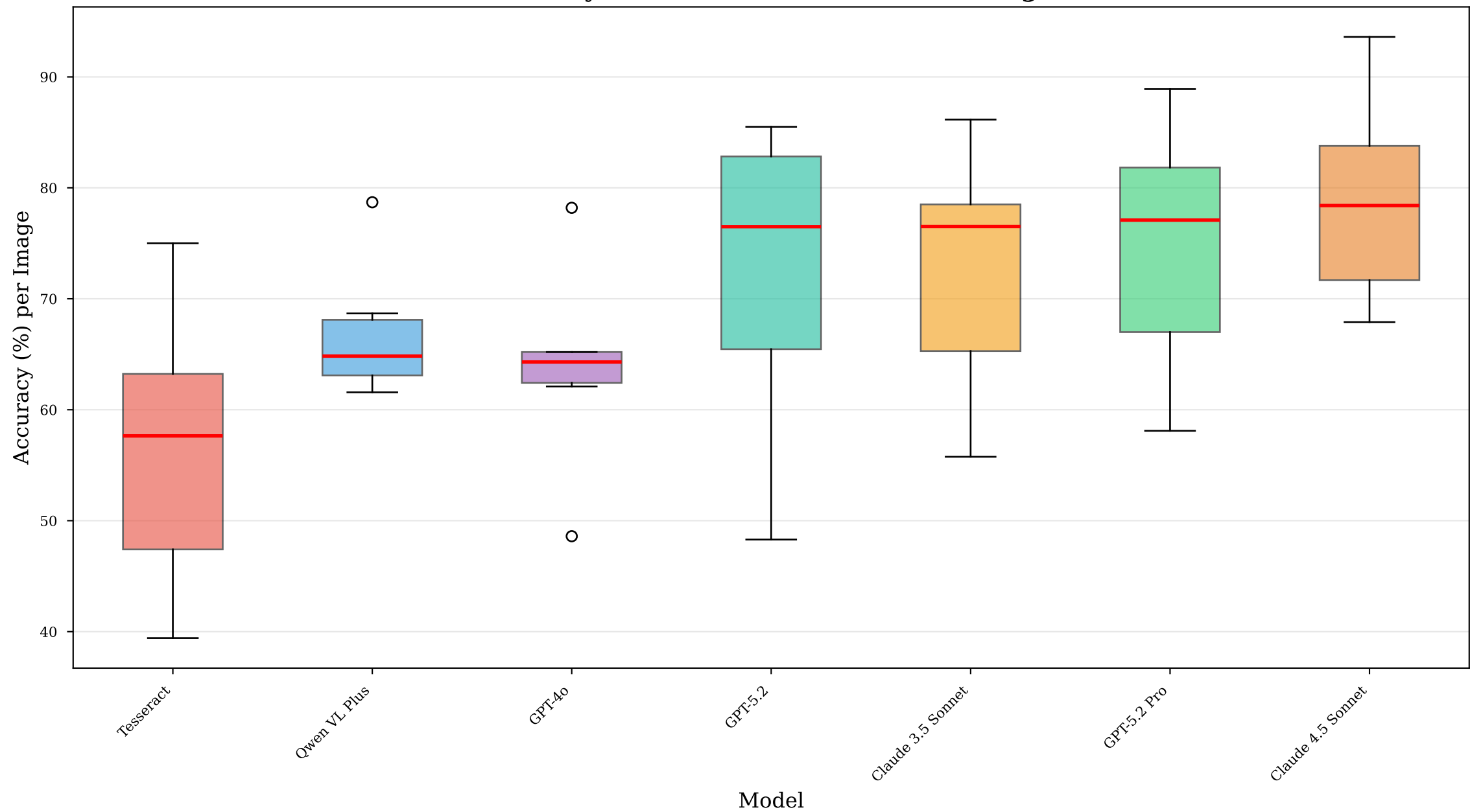
Accuracy Distribution Across 6 Test Images
