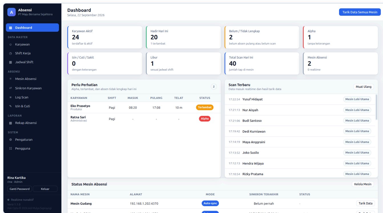
Gambar 3.1 — Dashboard
