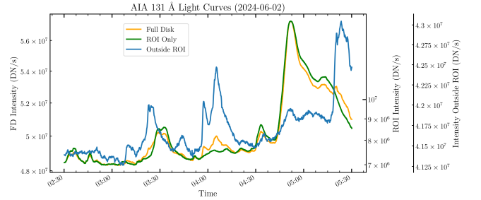
Figure C16. AIA 131 light curve
