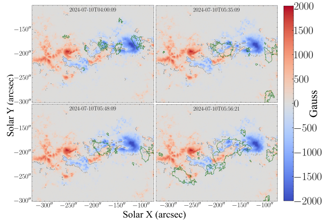
Figure 3. Case 4 HMI images, gray colour line represents PIL (0 Gauss value pixels) and green colour contours are SUIIT enhancement contours from difference image.
