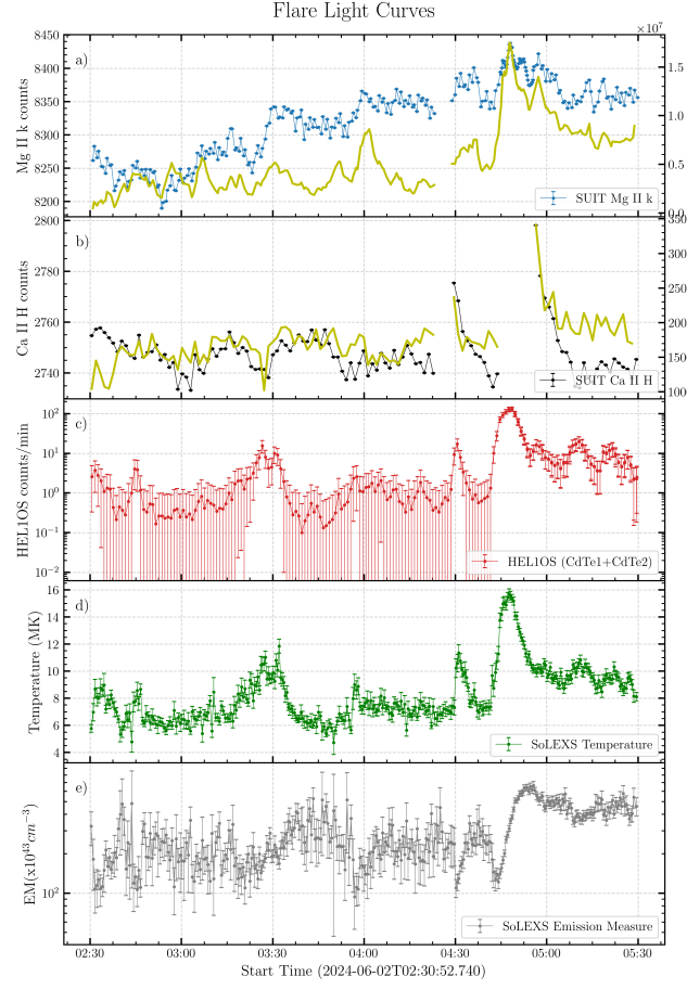
Figure C15. Case 2 light curves
