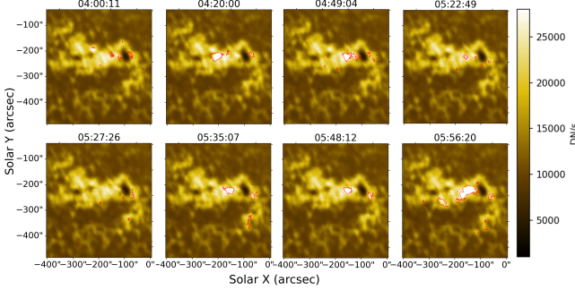
Figure 2. Case 4 : SUIIT time stamp images of pre-flare enhancements
