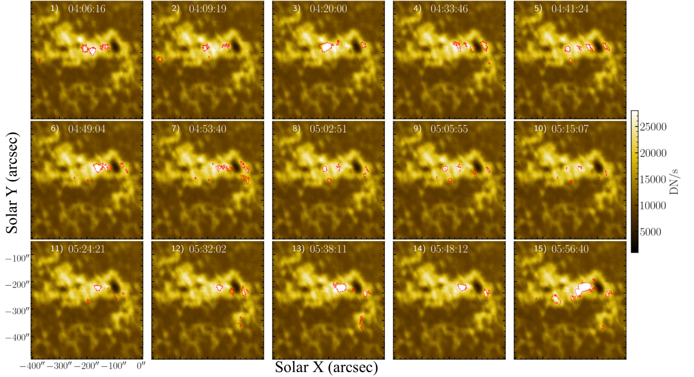
Figure A1. Case 4 timestamps
