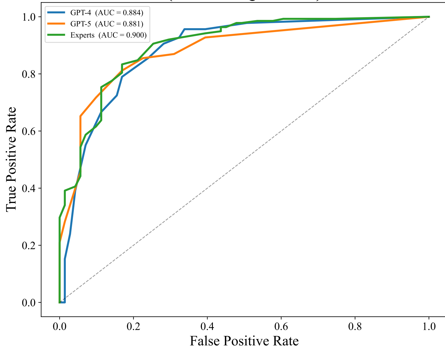
ROC Curve (label: PHQ-9 \geq 10 )
