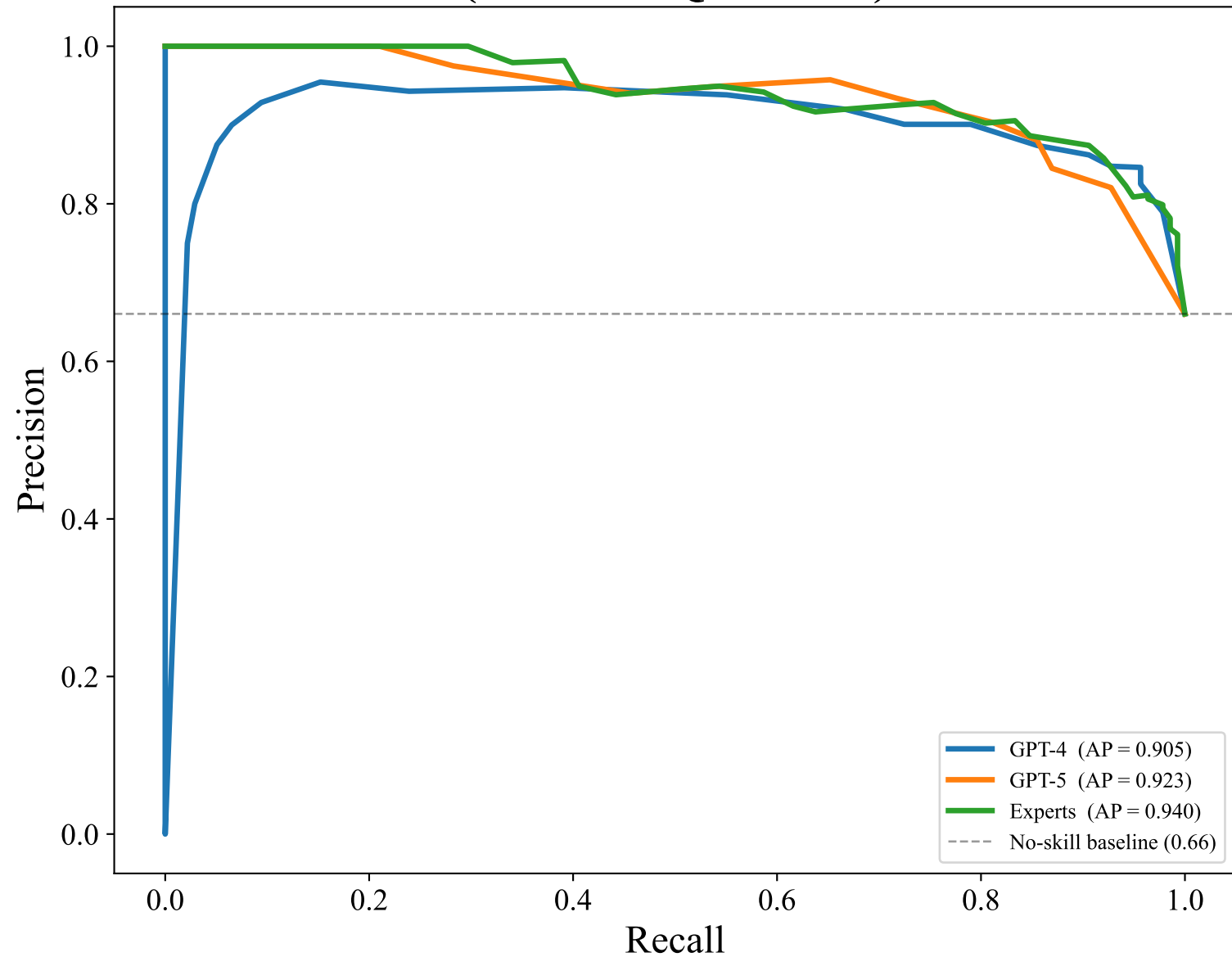
Precision-Recall Curve (label: PHQ-9 \geq 10 )
