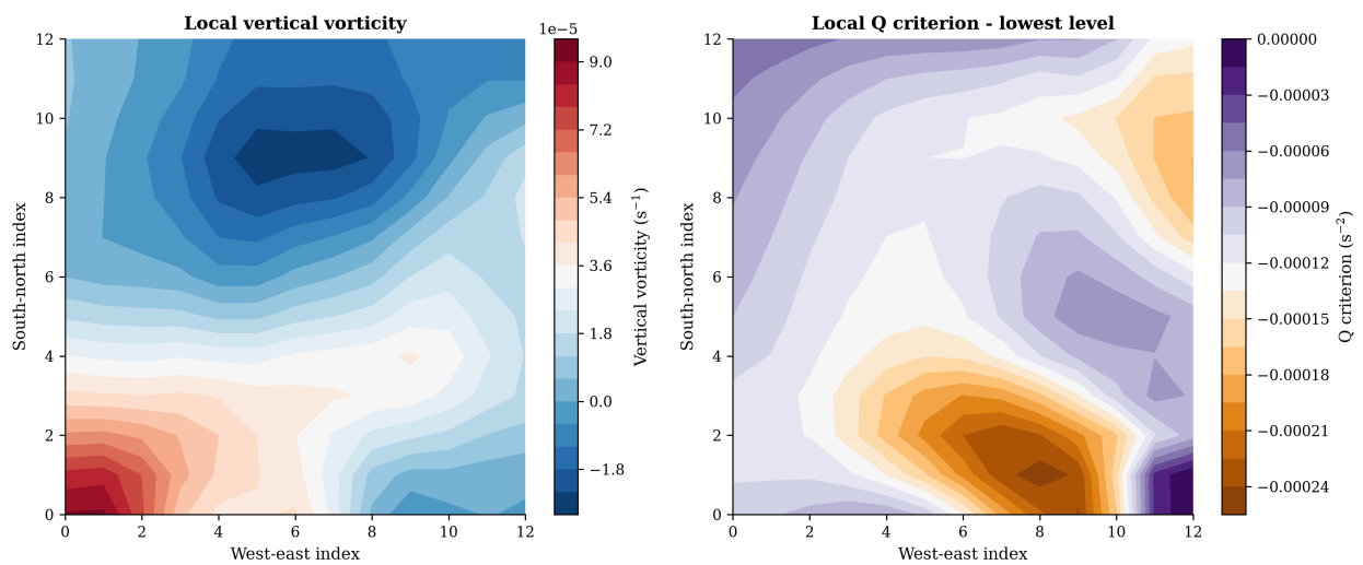
Flow Structure Diagnostics
