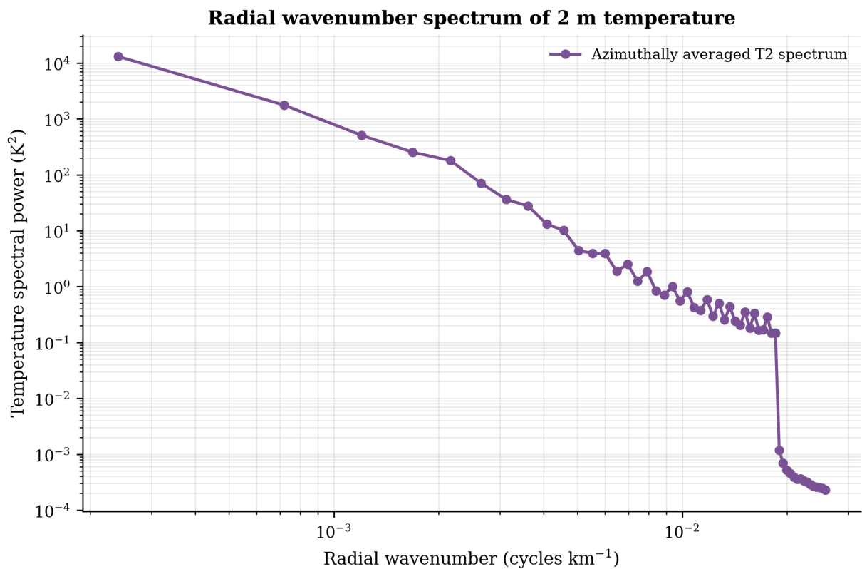
Temperature 2M Wavenumber Spectrum
