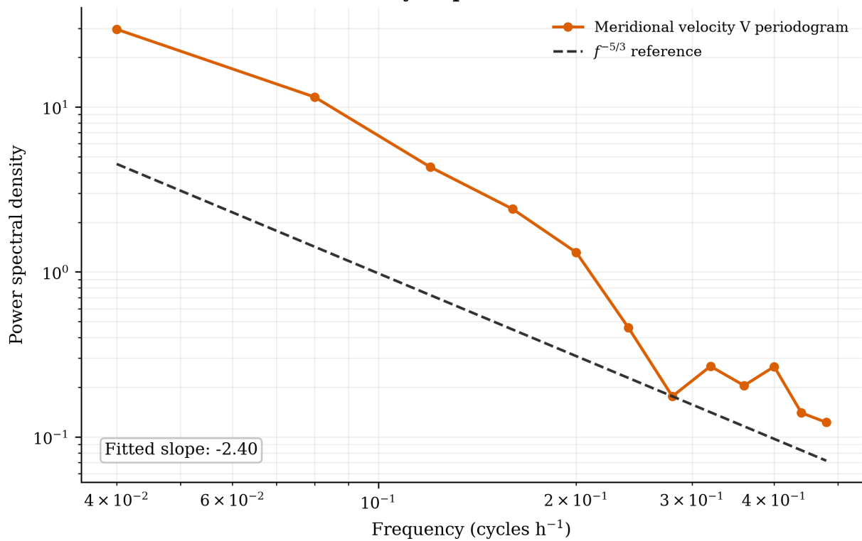
V Wind Spectrum
