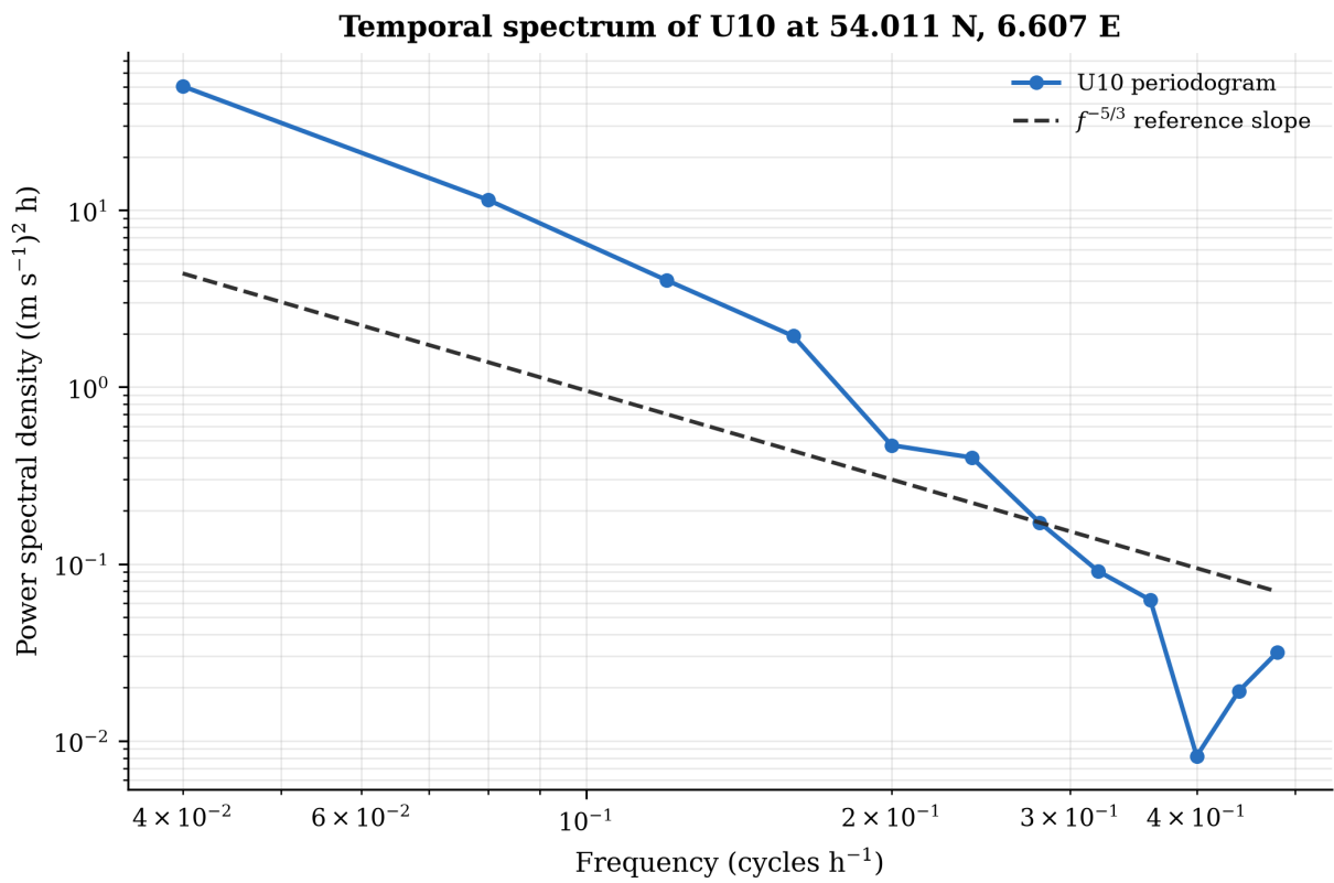
U10 Temporal Spectrum
