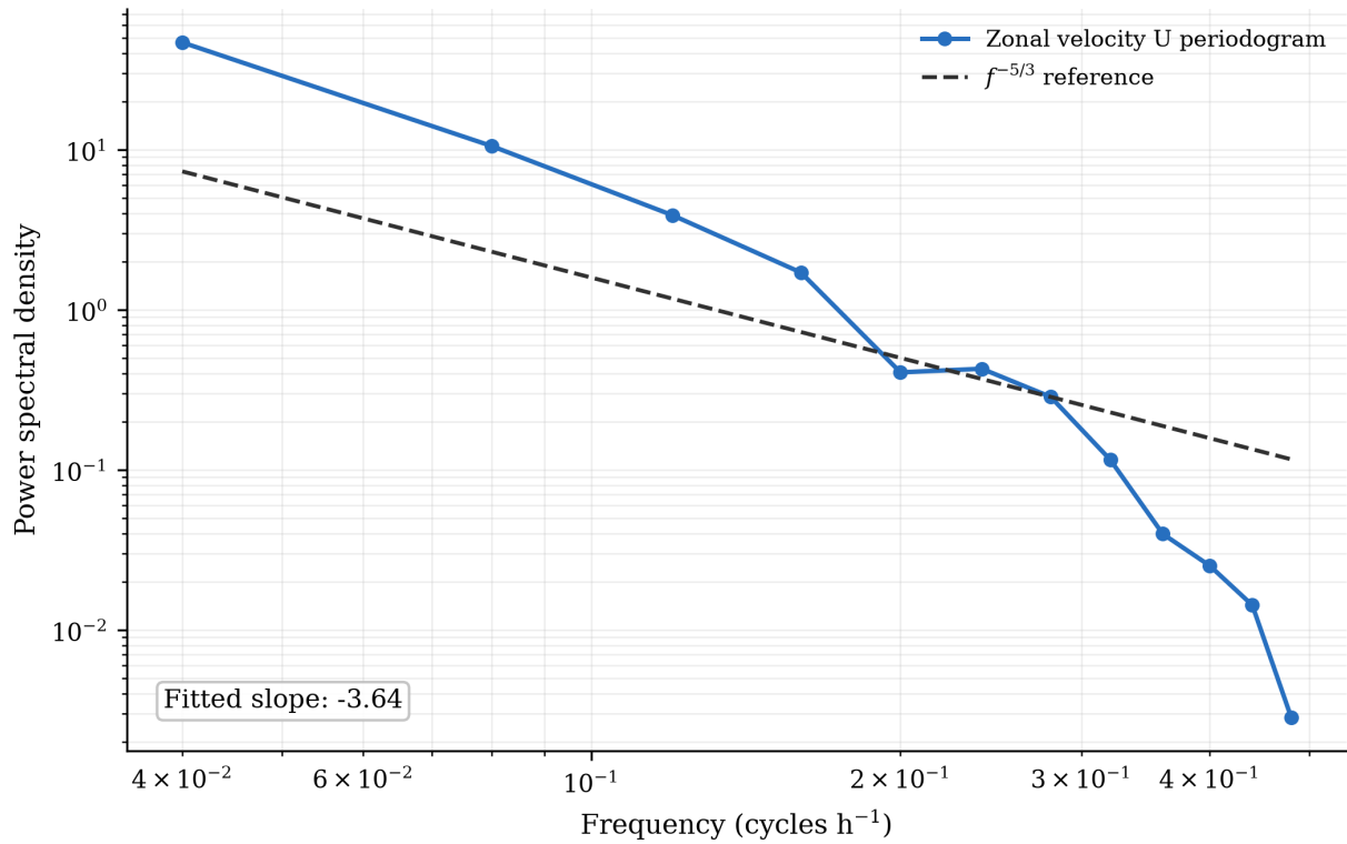
U Wind Spectrum
