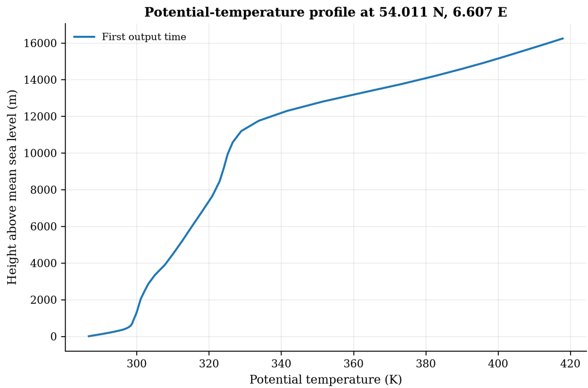
Potential Temperature Profile
