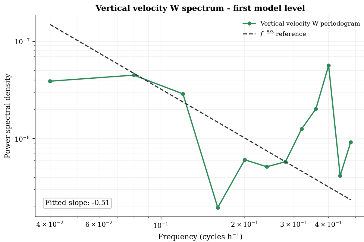
W Wind Spectrum
