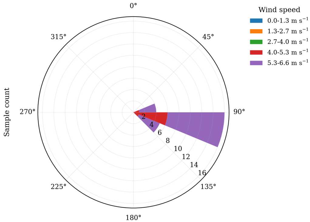
Wind Rose 10M
