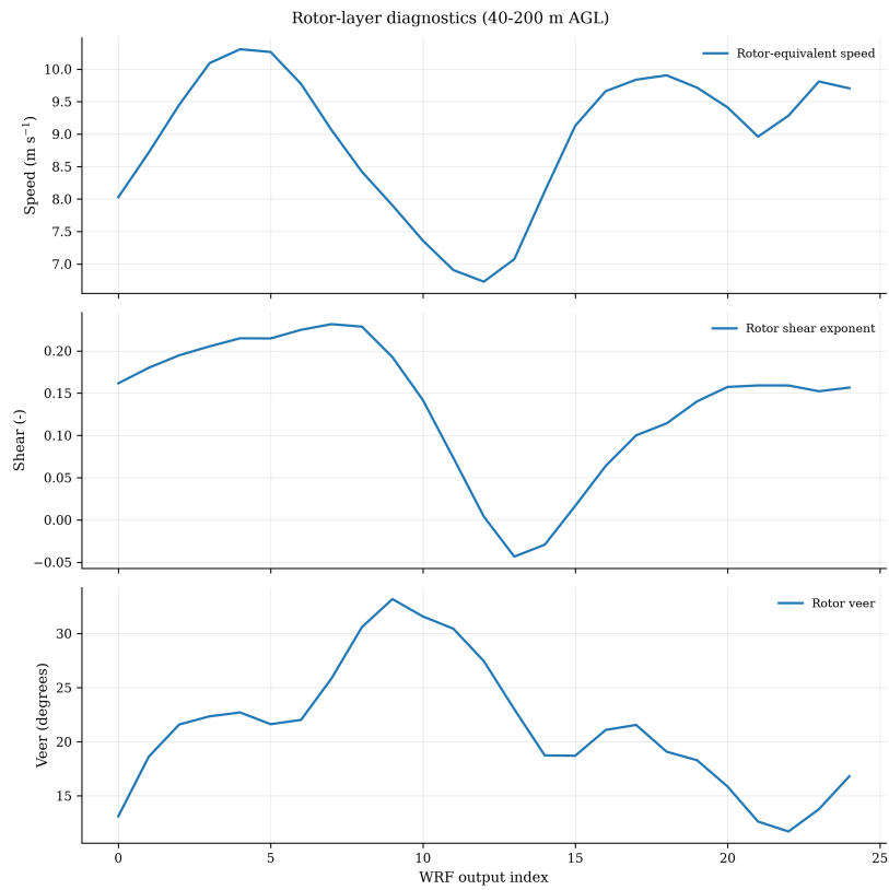
Rotor Diagnostics
