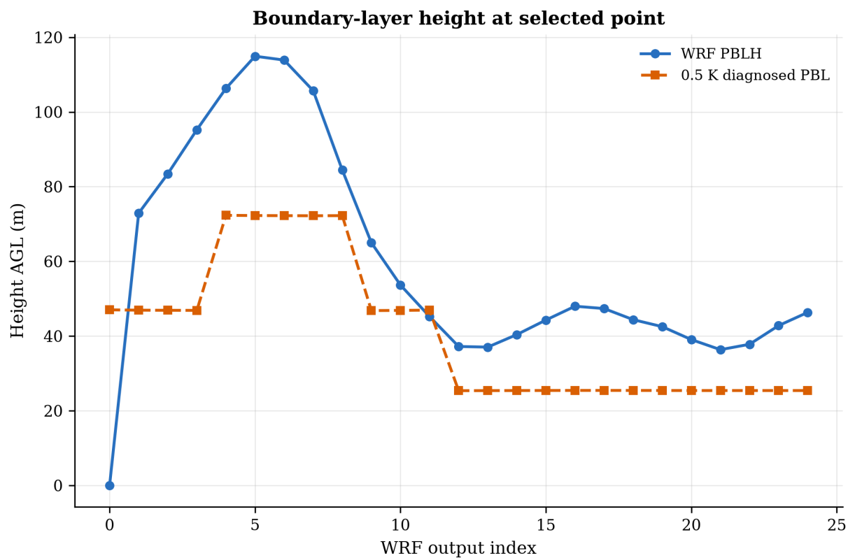
Boundary Layer Height
