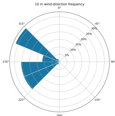
D02 Figure 4. Wind Rose.
