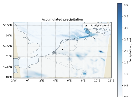
D01 Figure 5. Accumulated Precipitation.
