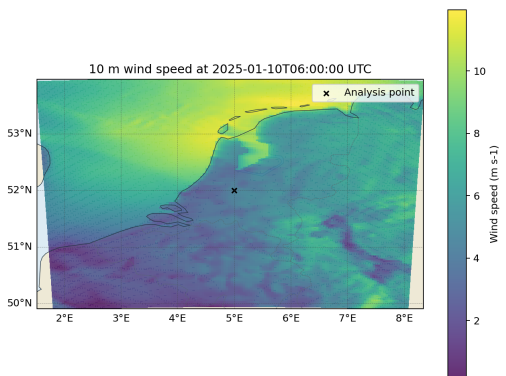
D02 Figure 3. Final Wind Speed.
