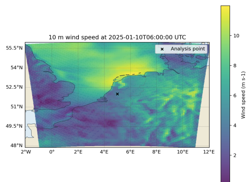
D01 Figure 3. Final Wind Speed.
