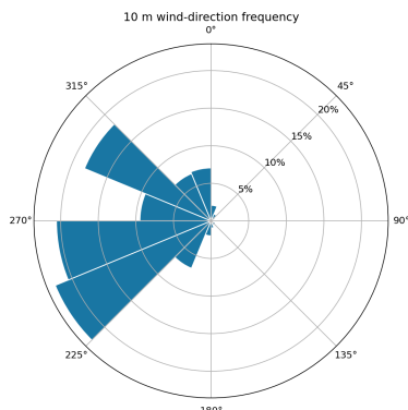
D01 Figure 4. Wind Rose.
