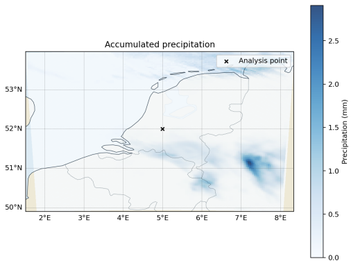
D02 Figure 5. Accumulated Precipitation.
