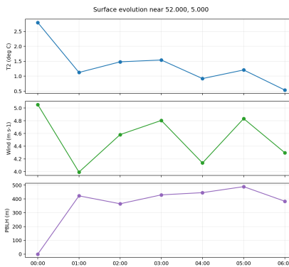
D01 Figure 6. Selected Point Timeseries.
