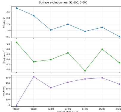
D02 Figure 6. Selected Point Timeseries.
