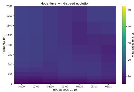
D02 Figure 9. Wind Time Height.
