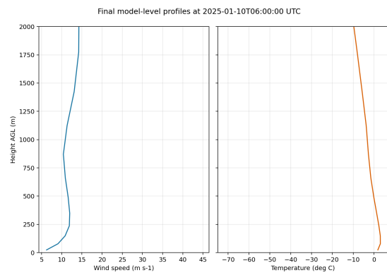
D02 Figure 8. Vertical Profiles.
