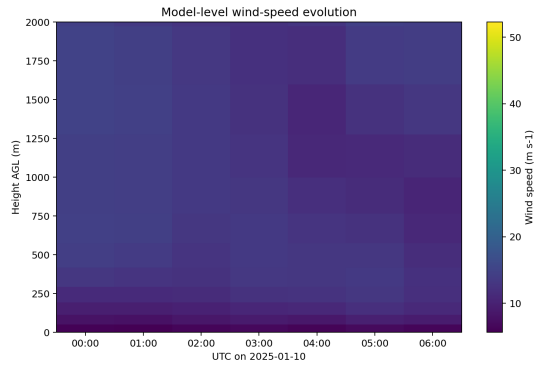
D01 Figure 9. Wind Time Height.
