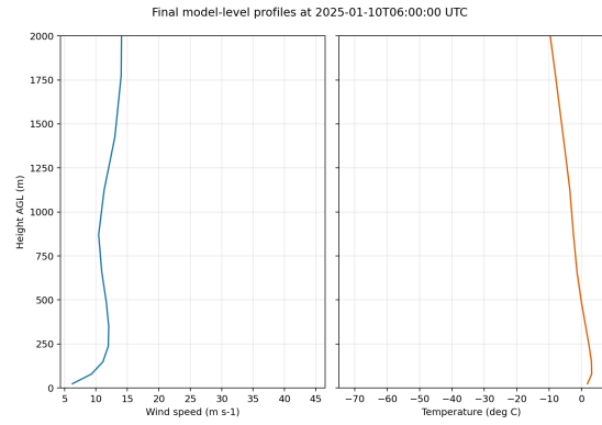
D01 Figure 8. Vertical Profiles.
