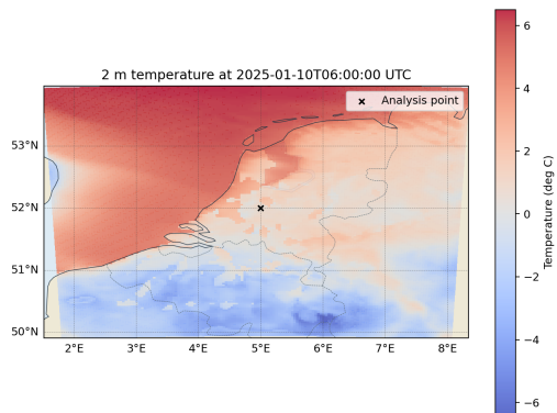
D02 Figure 2. Final Temperature.
