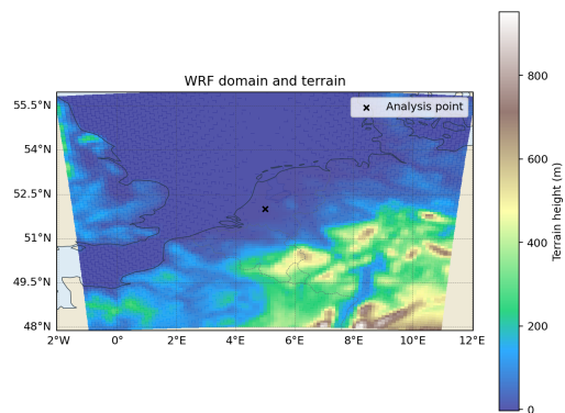
D01 Figure 1. Domain Terrain.
