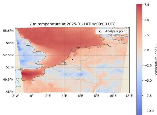
D01 Figure 2. Final Temperature.
