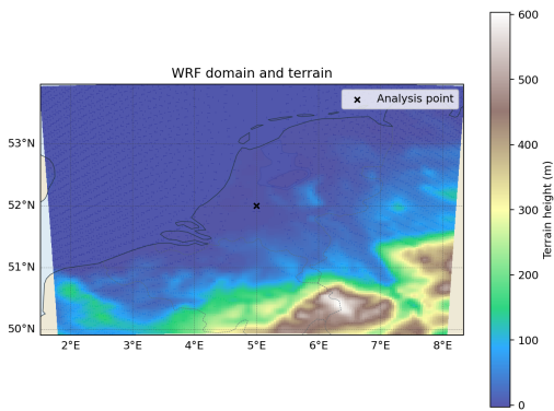
D02 Figure 1. Domain Terrain.
