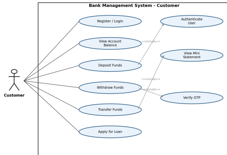
Figure 1: Use-case diagram - Customer interactions with the Bank Management System.
