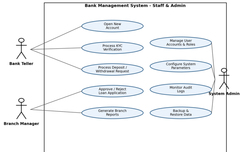
Figure 2: Use-case diagram - Bank Teller, Branch Manager, and System Administrator interactions.
